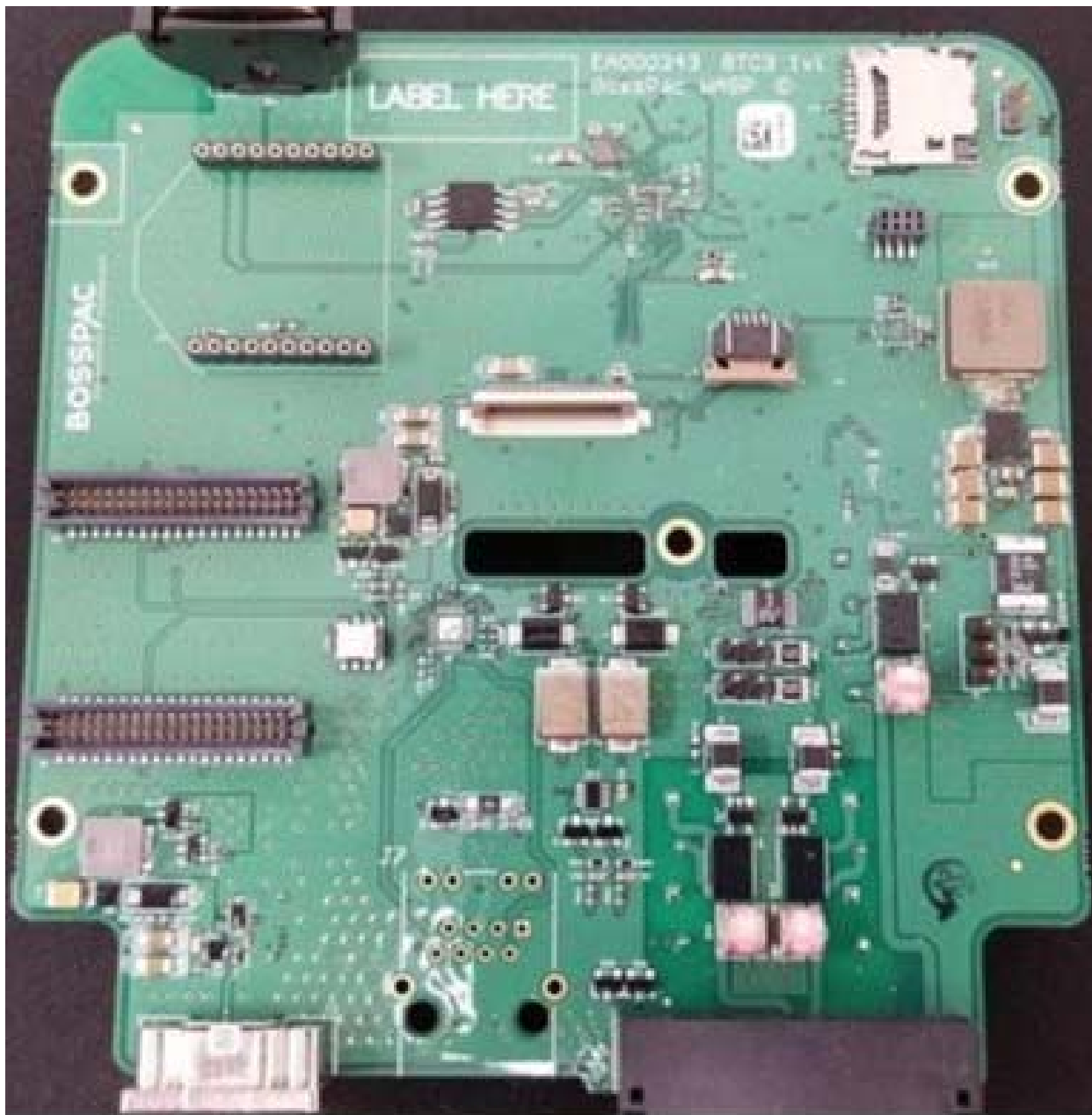
Figure E11A.1 – Internal, NEST4, PCB Top
