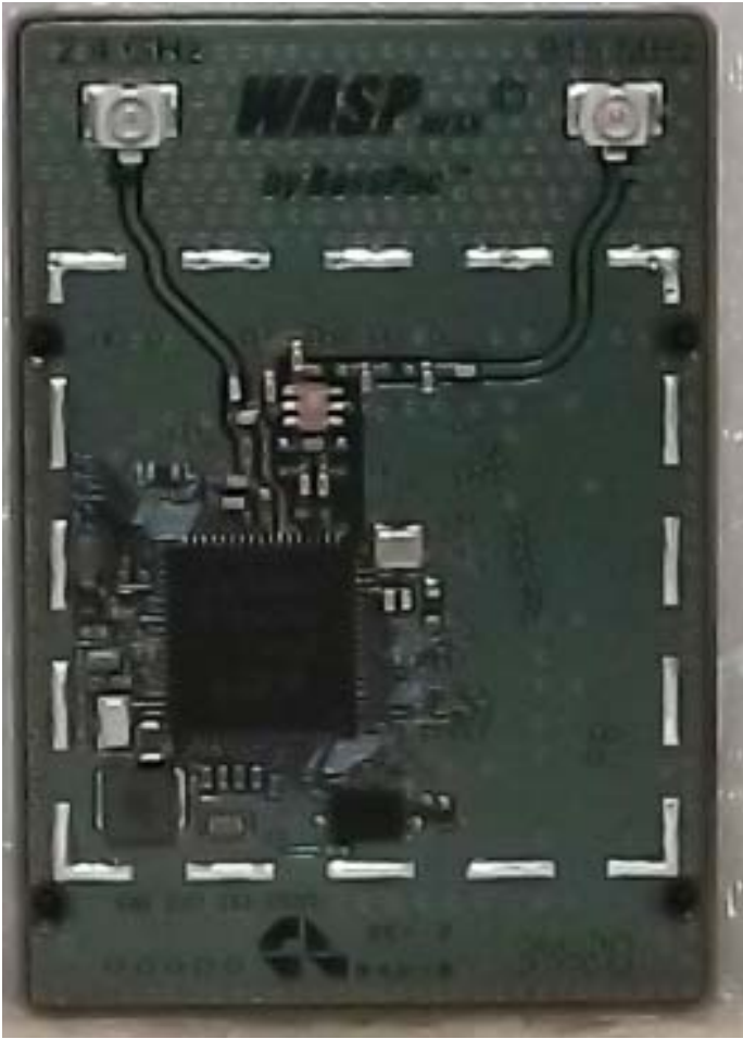
Figure E22.3 – Module Top, Shield Removed
