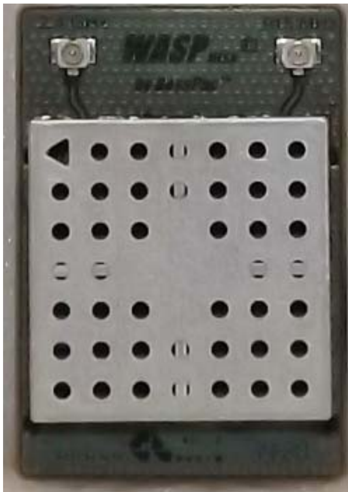
Figure E22.1 – Module Top
