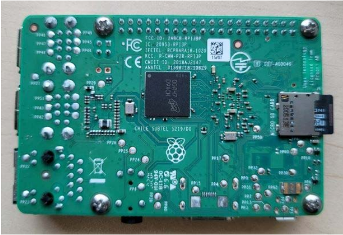
Figure E23.5 – Internal, Bottom PCB, Bottom
