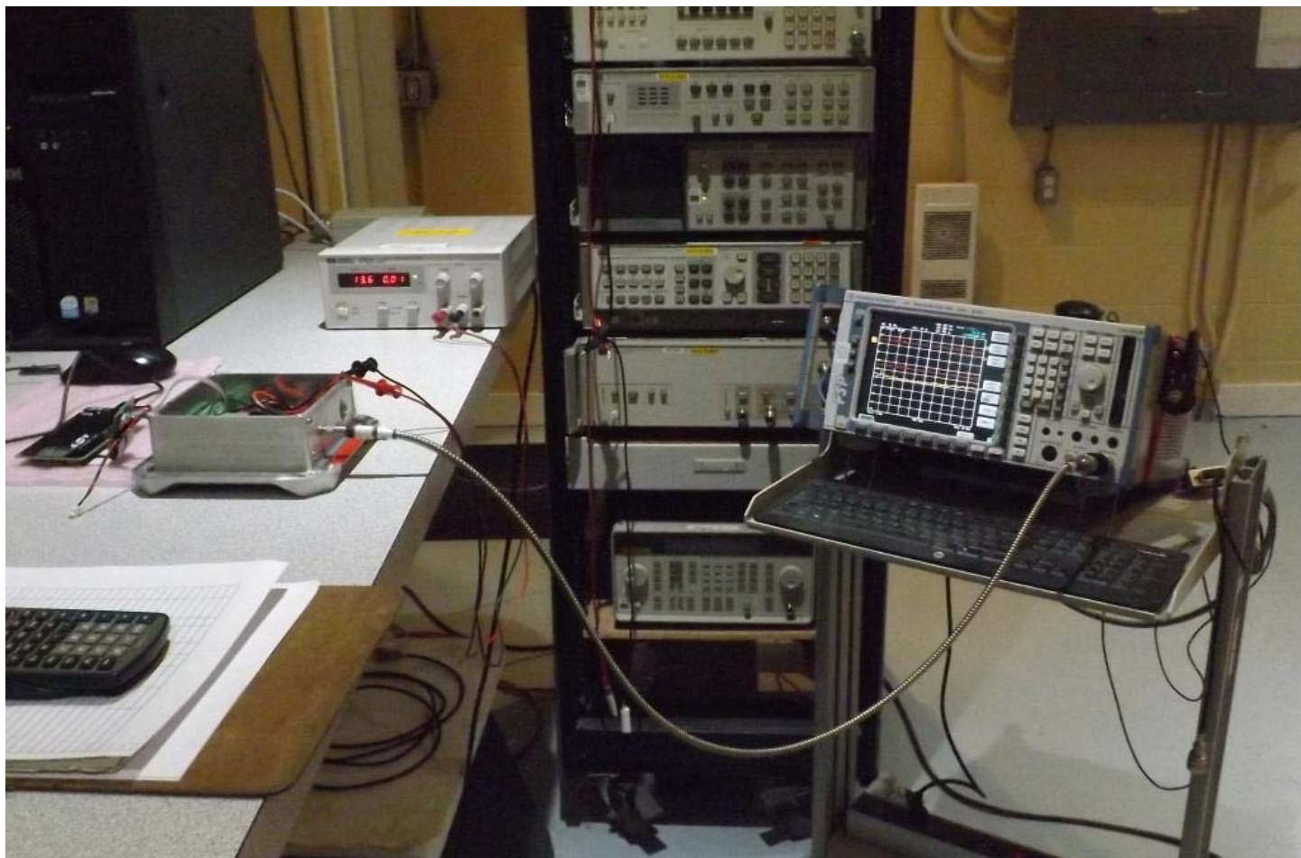
Figure E25.1 – Conducted Measurements
