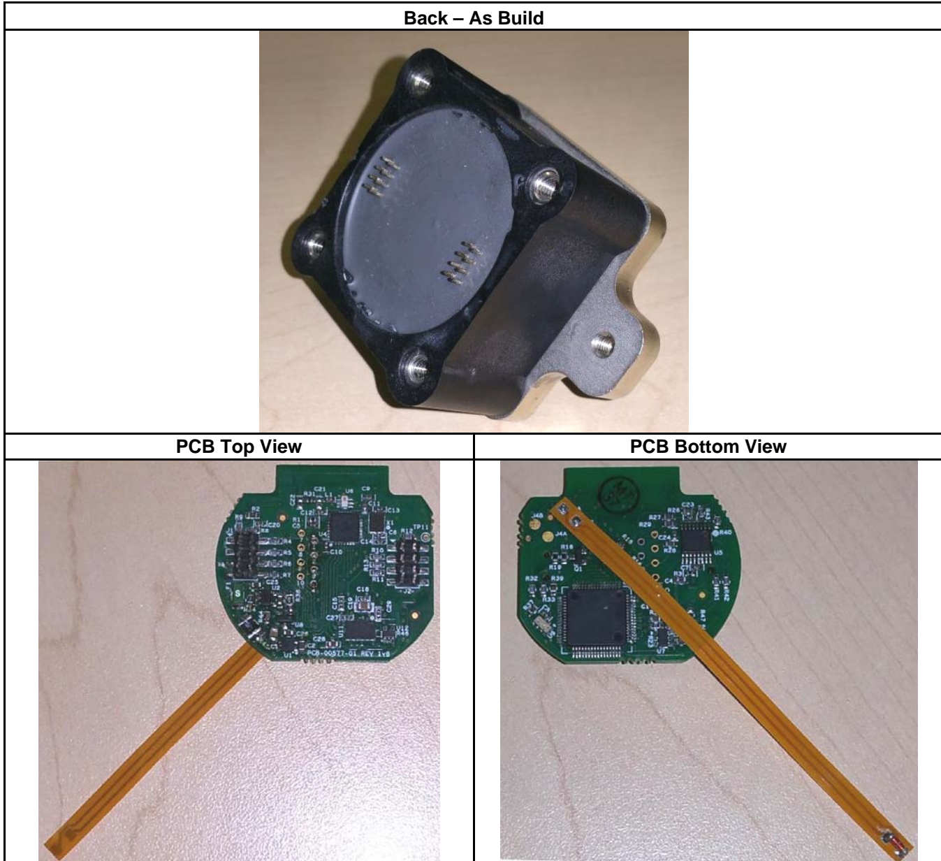
Figure 1 Internal Photos
