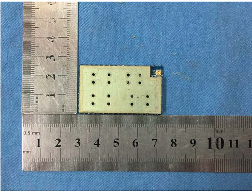
Reversed polarity non standard external antenna port
