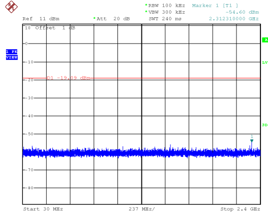
Modulation Type: \pi/4 DQPSK (2Mbps) CH19
