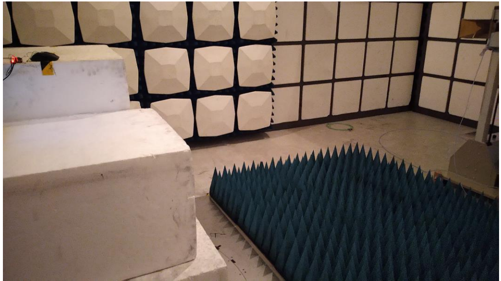
Side view
