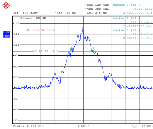
20dB Bandwidth CH01, 2402MHz
