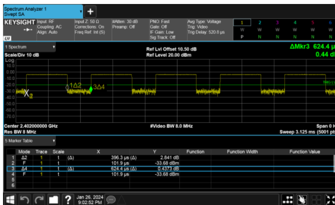
Modulation Type: GFSK(2Mbps)
