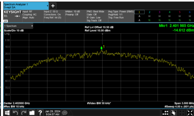
Modulation Type: GFSK(2Mbps) CH00
