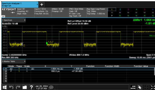
Modulation Type: GFSK (DH3) Channel: 00
