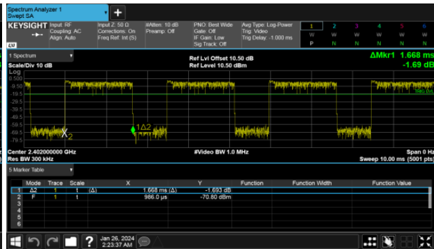
Modulation Type: \pi/4 -DQPSK (DH3) Channel: 00
