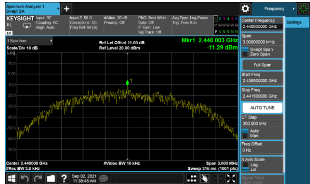
Modulation Type: GFSK(2Mbps) CH19
