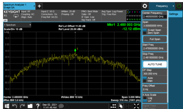
Modulation Type: GFSK(2Mbps) CH39
