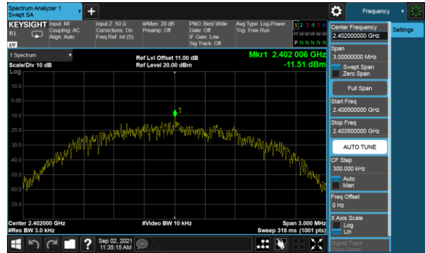
Modulation Type: GFSK(2Mbps) CH00
