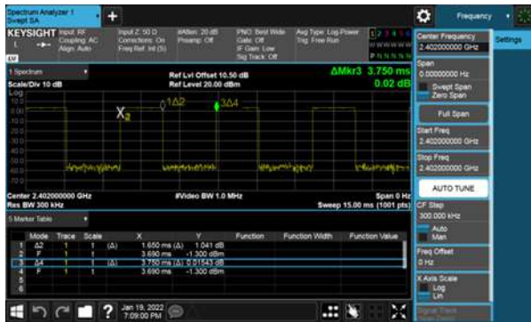
Modulation Type: GFSK-DH3 Channel: 00
