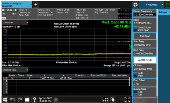
Modulation Type: \pi/4 -DQPSK, CH01
