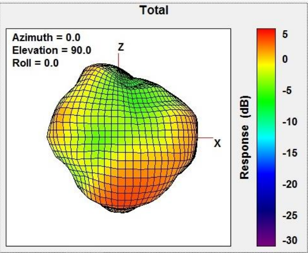
Total Gain Back Face view 2483.5MHz
