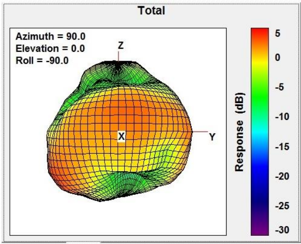
Total Gain Left Side view 2400MHz
