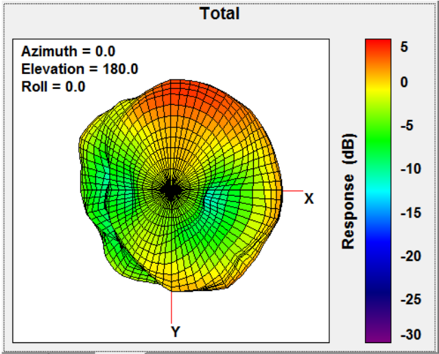
Total Gain Bottom view 2440MHz
