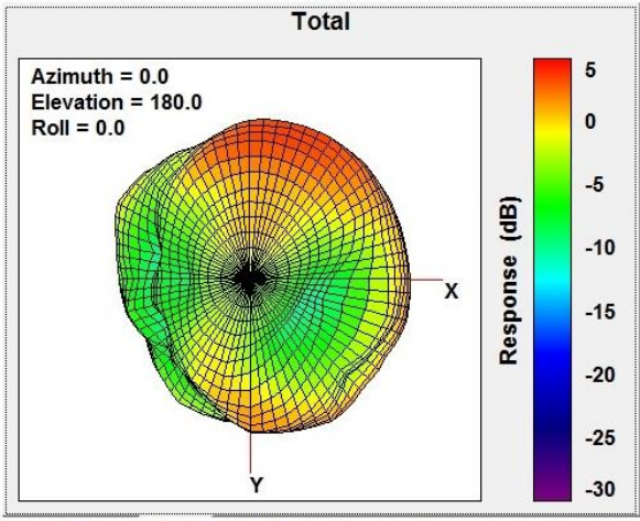
Total Gain bottom view 2400MHz
