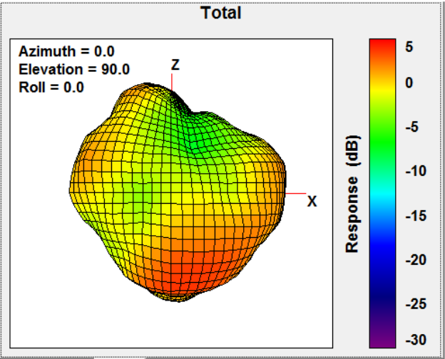
Total Gain Back Face view 2440MHz
