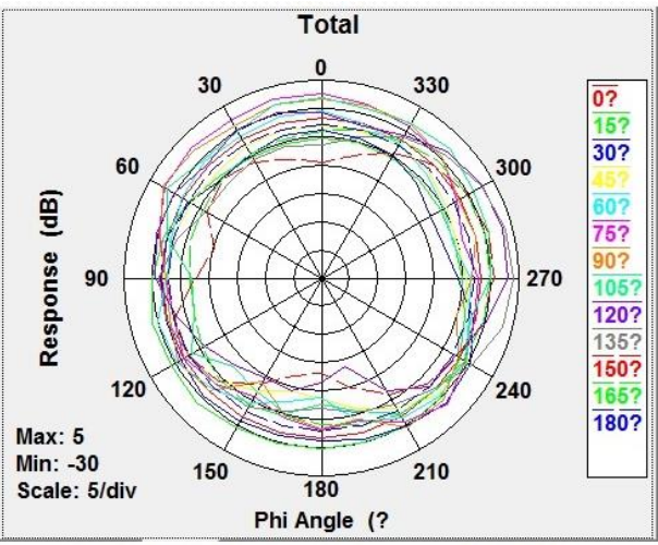
Total Gain Right Side view 2483.5MHz
