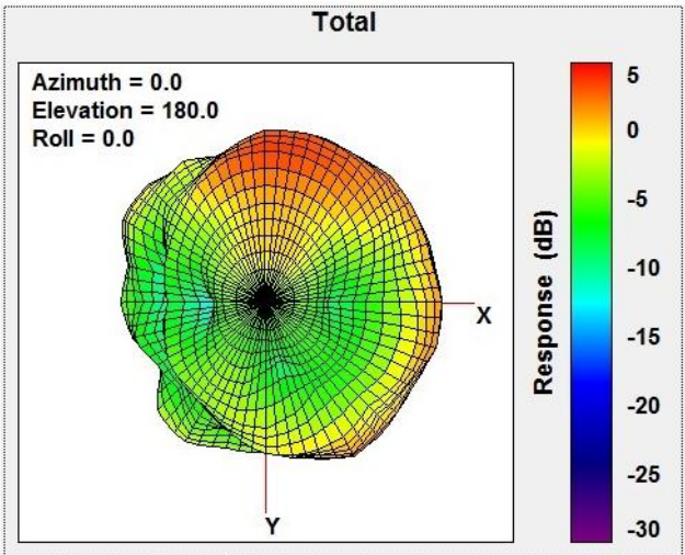
Total Gain Bottom view 2483.5MHz
