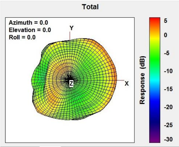
Total Gain Top view 2483.5MHz
