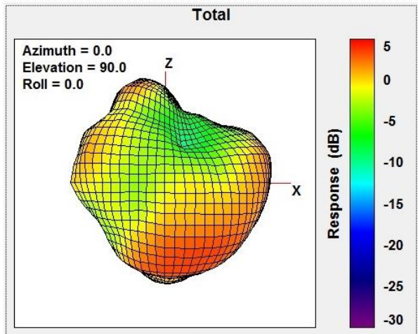
Total Gain Back Face view 2400MHz
