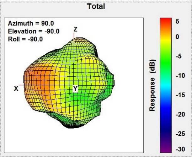
Total Gain Front Face view 2483.5MHz
