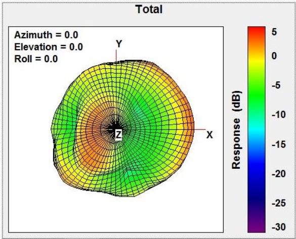
Total Gain Top view 2400MHz
