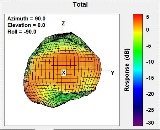
Total Gain Left Side view 2483.5MHz
