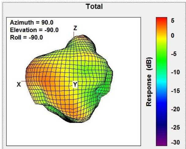
Total Gain Front Face view 2400MHz
