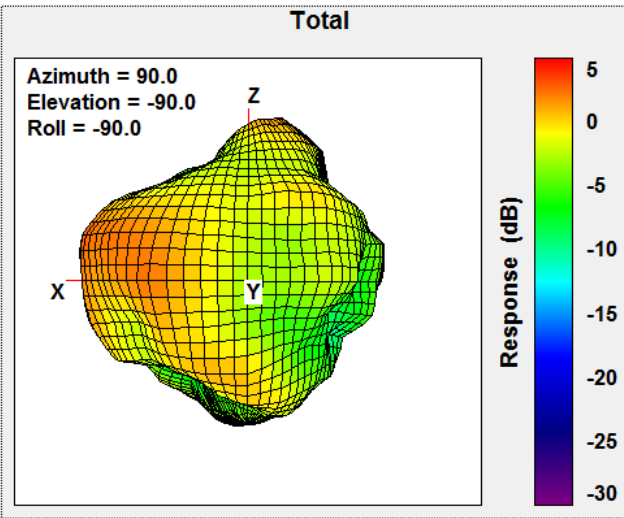
Total Gain Front Face view 2440MHz
