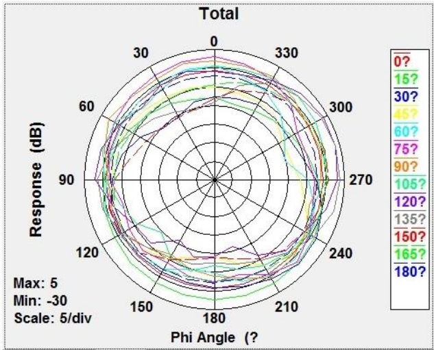
Total Gain Right Side view 2400MHz
