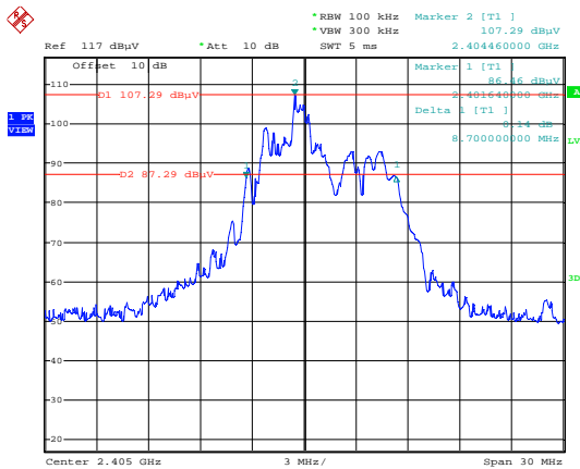
20dB Bandwidth CH01, 2405MHz
