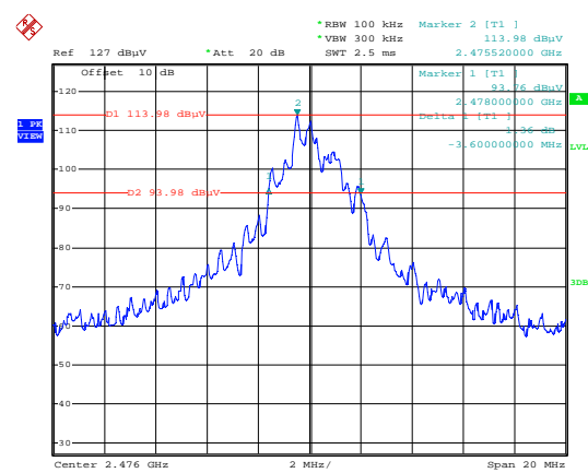
CH16, 2476MHz
