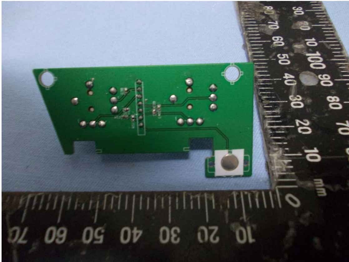
12 Rear view of PCB 02
