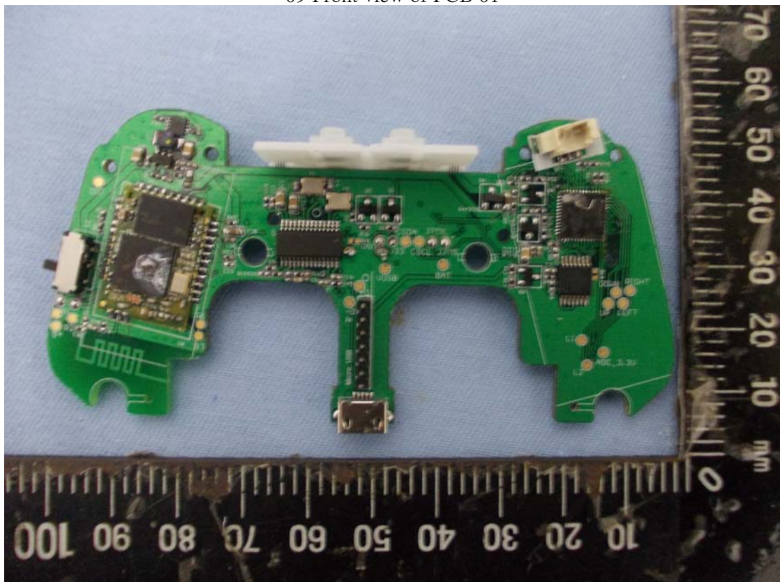
09 Front view of PCB 01
