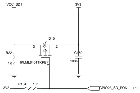
SD CARD
