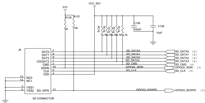
SD CARD
