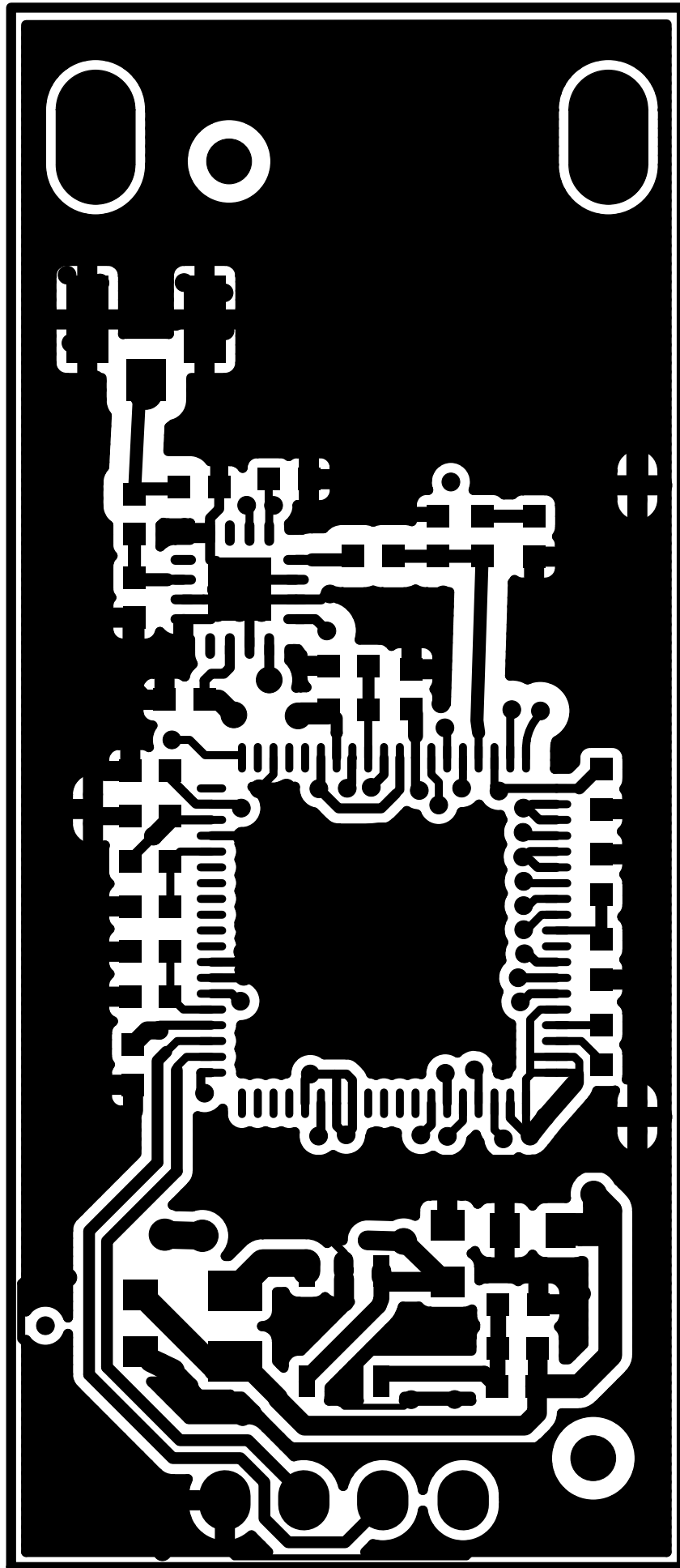
TopLayer
