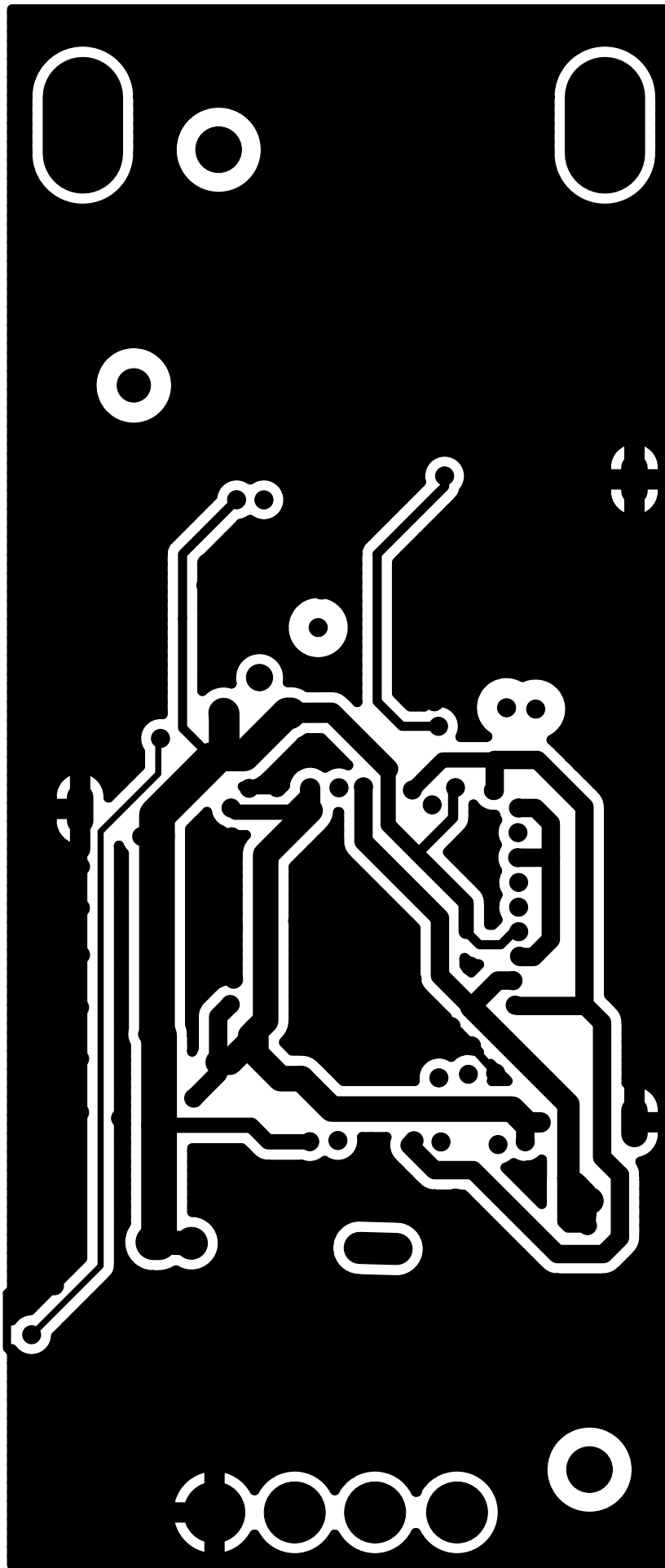
MidLayer2
