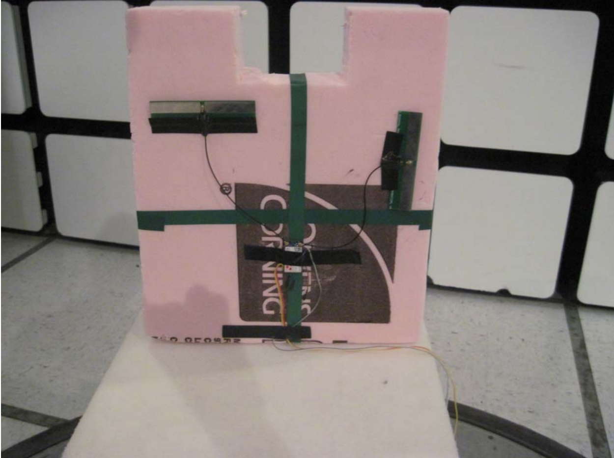
Radiated Measurements in Semi-Anechoic Chamber
