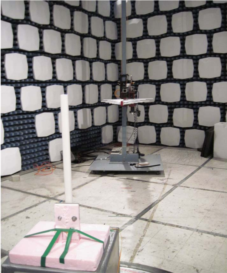
Radiated Measurements in Semi-Anechoic Chamber
