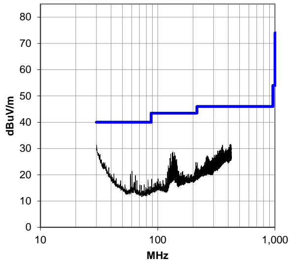
Omni, Mid Ch: 30-425 MHz, Run 162
