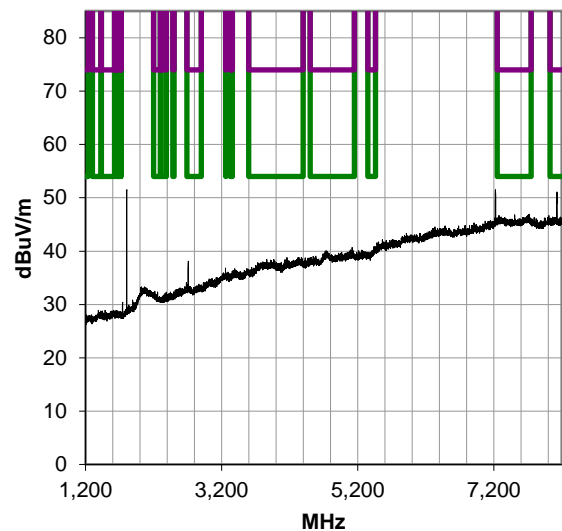
Internal Antenna, Low Ch: 1200-8200 MHz, Run 113
