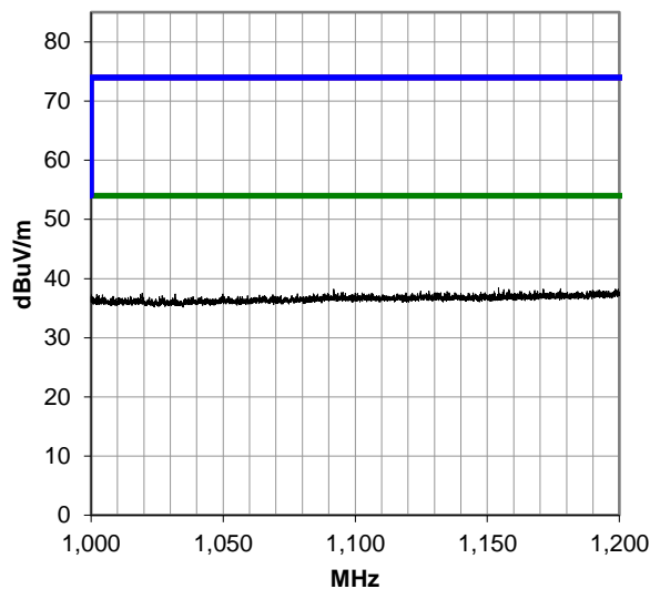
Internal Antenna, Low Ch: 1000-1200 MHz, Run 120
