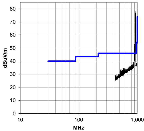
Yagi, High Ch: 425-1000 MHz, Run 157
