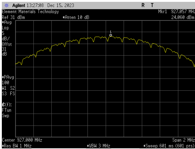
LoRa, Spreading Factor = 8, 500 kHz BW, Coding Rate =4/8 Internal Antenna Port High Ch = 927 MHz
