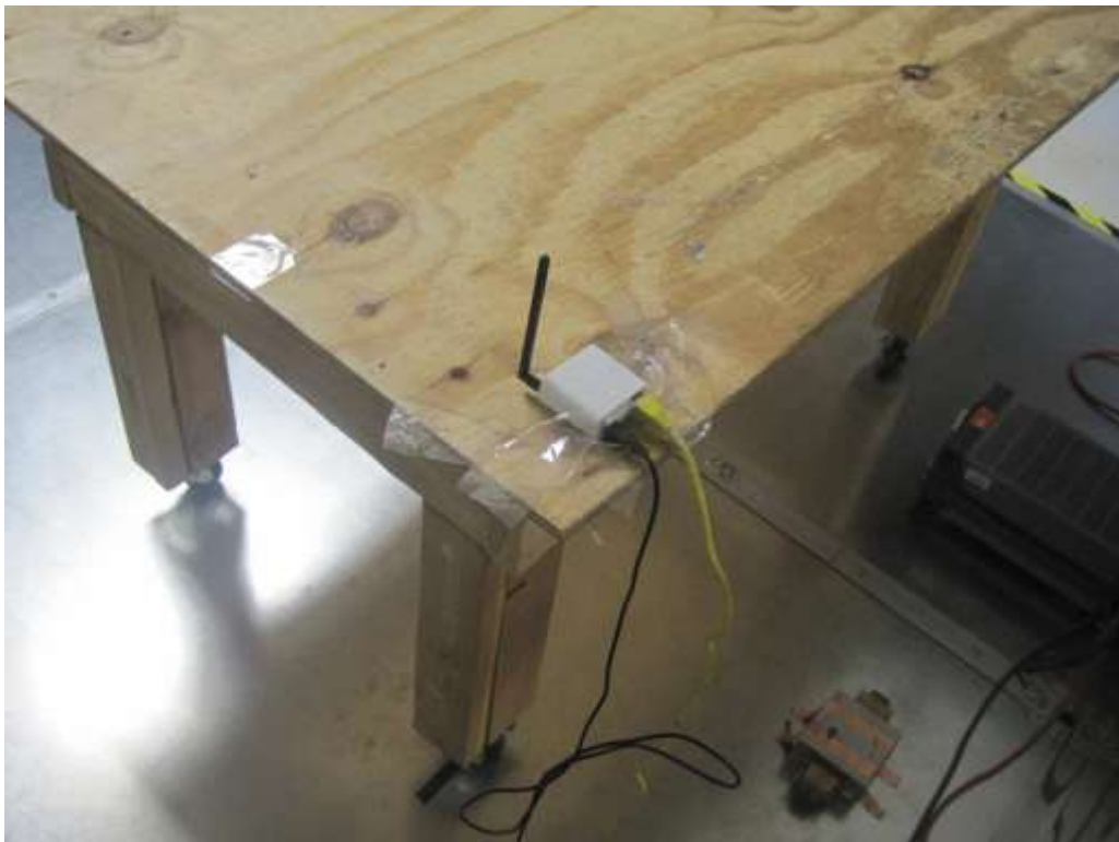
AC Line Conducted Emission Set up - Front View
