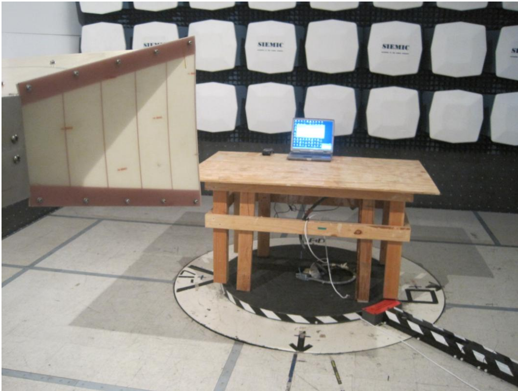
Radiated Emission (1 GHz – 5 GHz) – Front View
