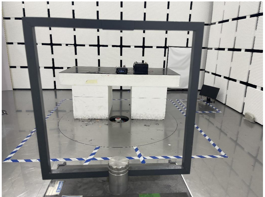
sRadiation Emission Test Setup (Below 30MHz)
