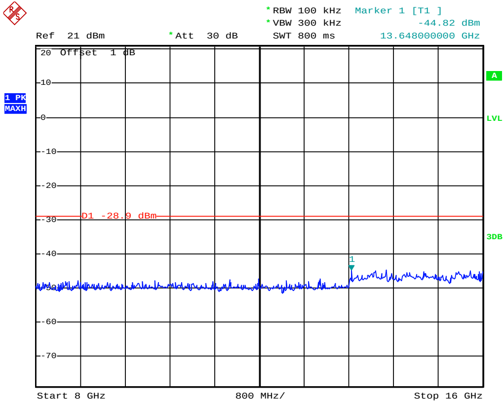
(Plot 4.6.4 A2: Channel 3: 2422MHz @ 802.11n(40MHz))
