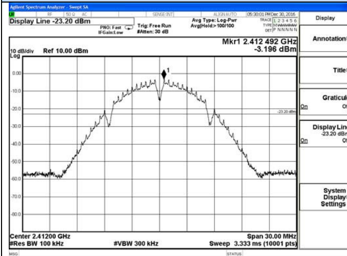
802.11b Low channel Reference
