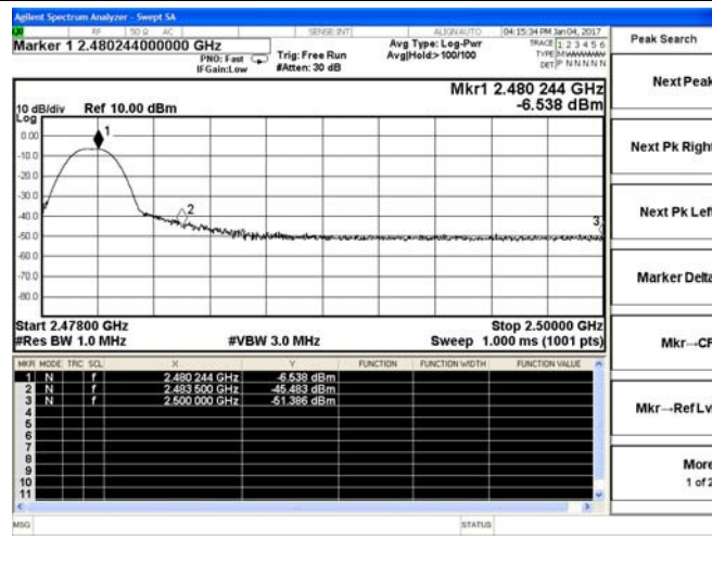
BLE 4.0-High channel(Peak)
