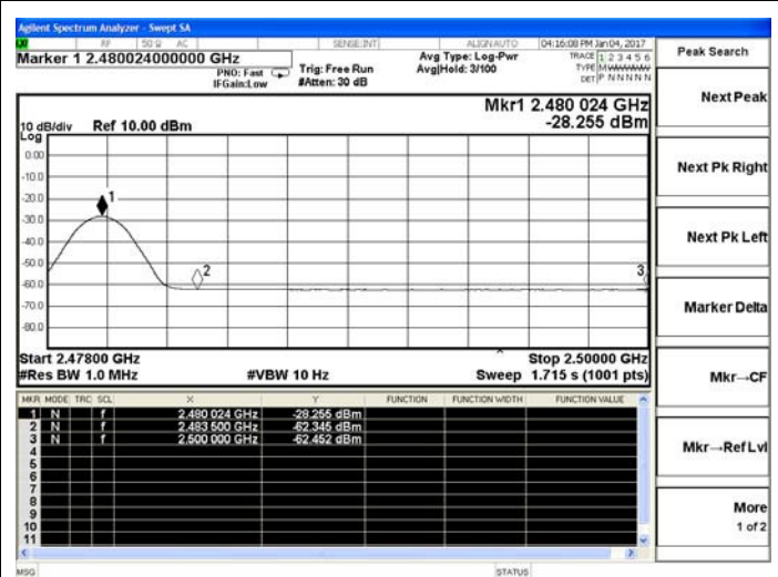
BLE 4.0-High channel(Average)
