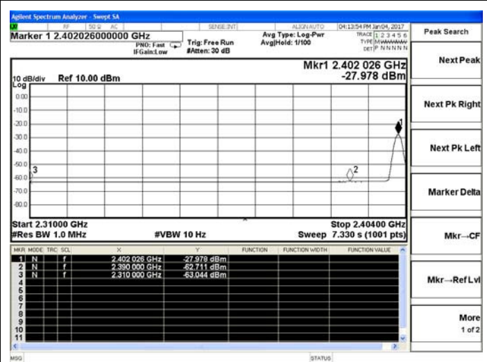
BLE 4.0-Low channel(Average)
