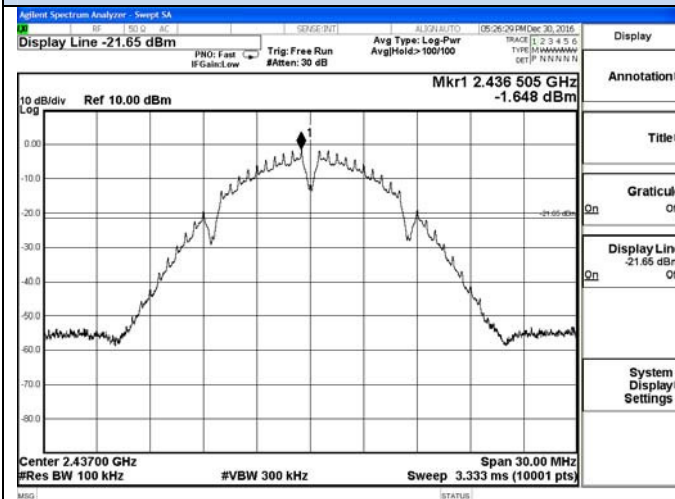
802.11b Middle channel Reference
