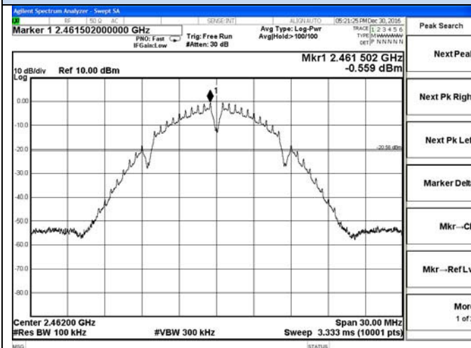
802.11b High channel Reference
