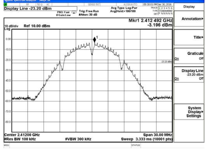
802.11b_Low Channel
