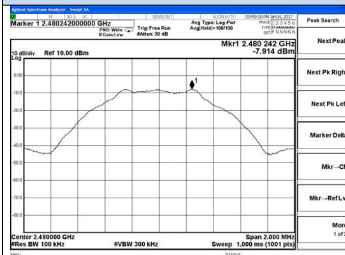
BLE 4.0-High channel Reference
