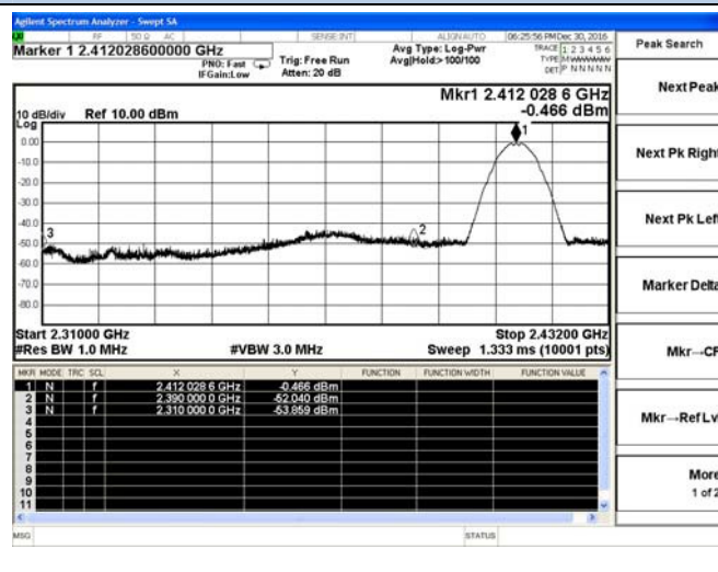
802.11b Low channel(Peak)
