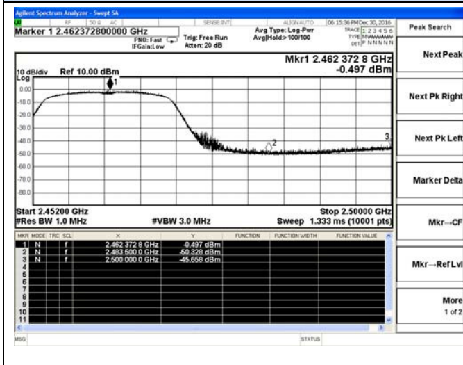
802.11n-HT20 High channel(Peak)
