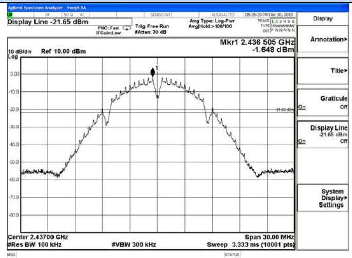
802.11b_Middle Channel
