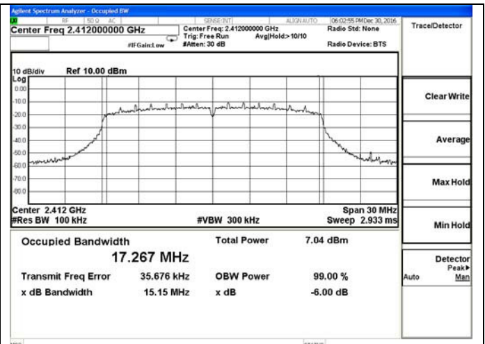
802.11n-HT20 Low channel
