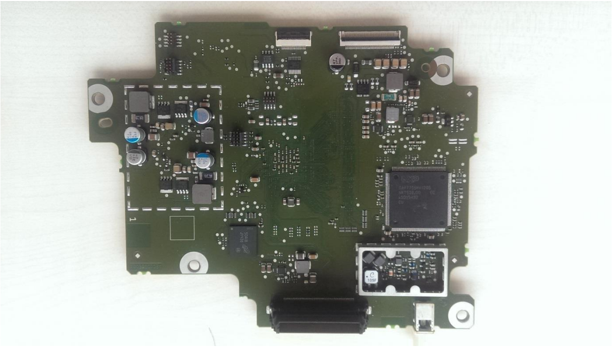
Bottom View of SoC PCB
