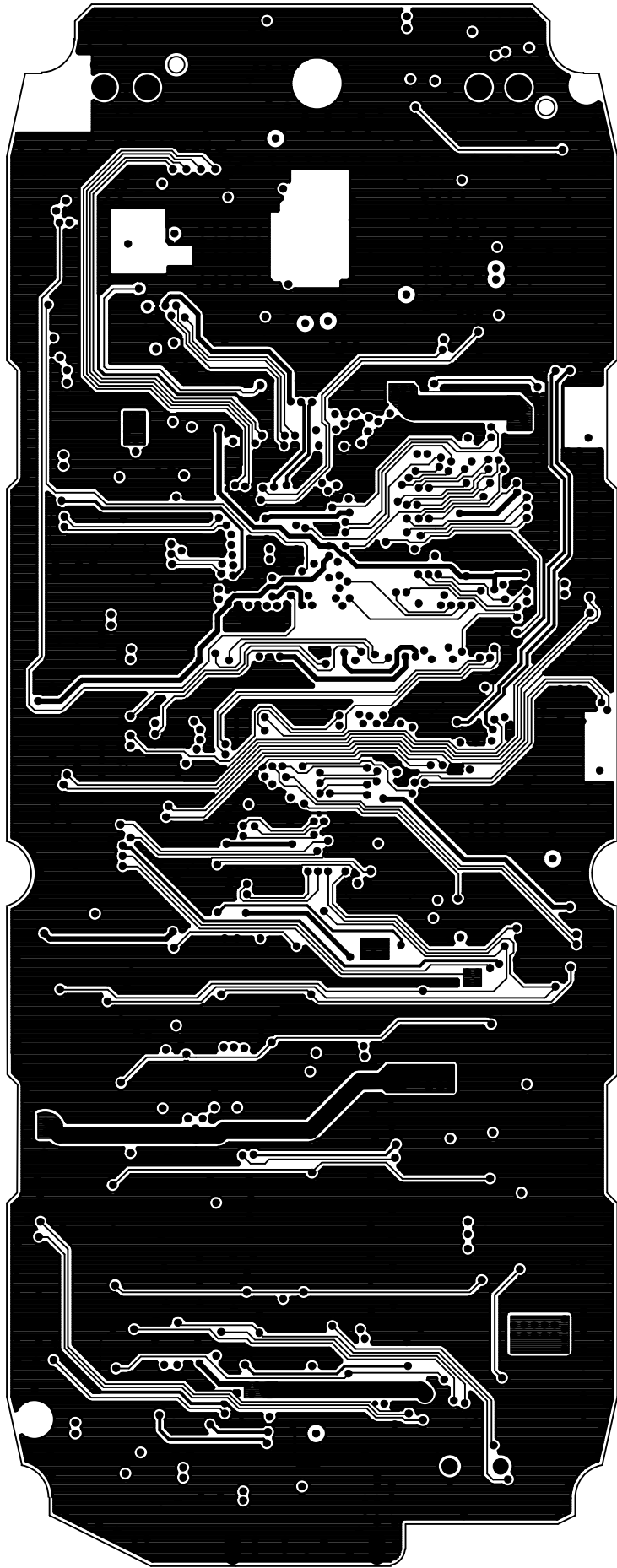
Layer2 routing
