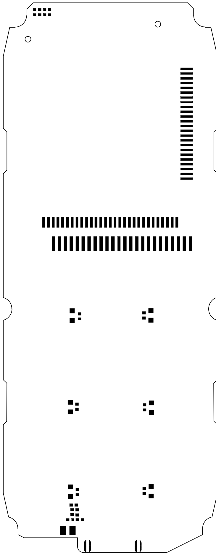
Paste mask Bottom
