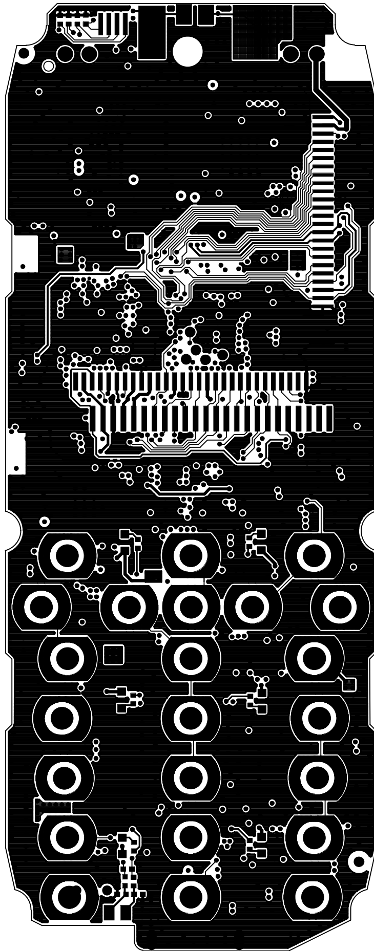
Bottom routing
