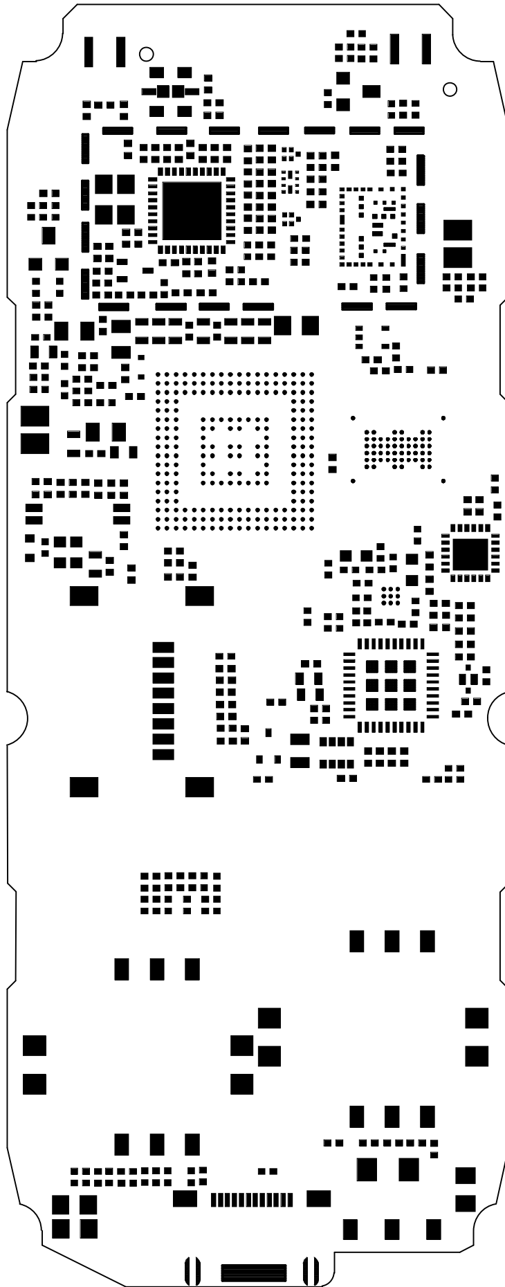
Paste mask Top
