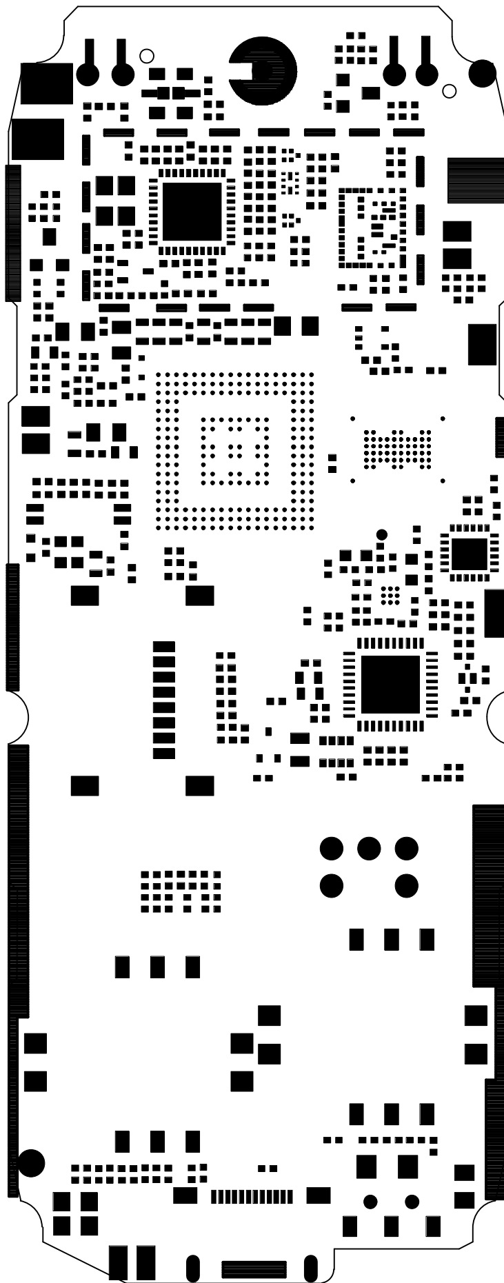
Solder mask Top
