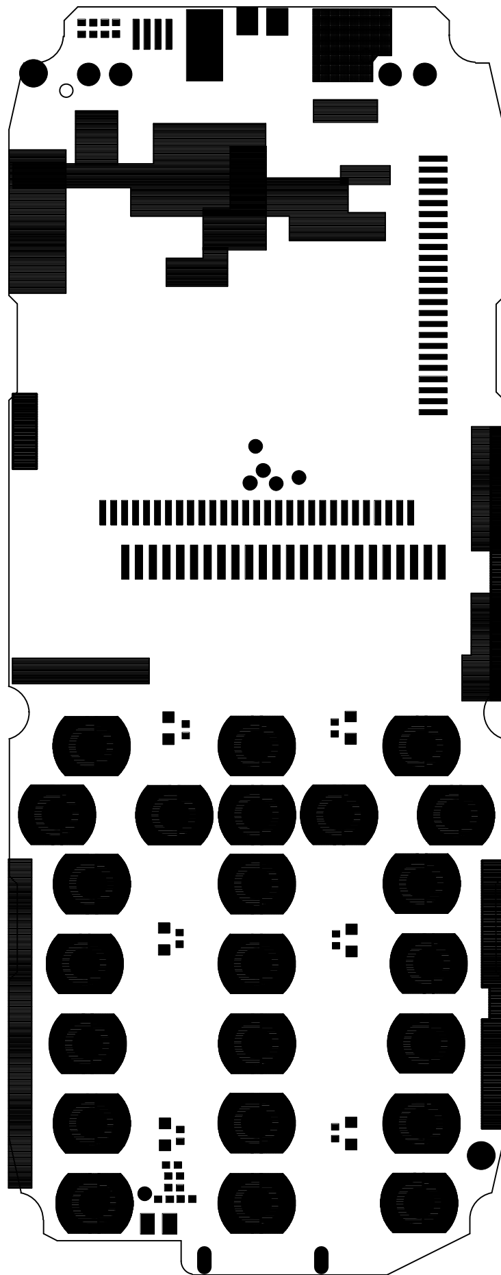
Solder mask Bottom
