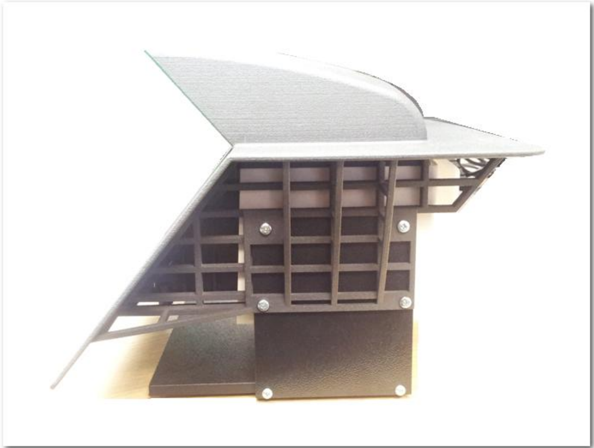
SIDE VIEW – MOUNTED IN TEST FRAME
