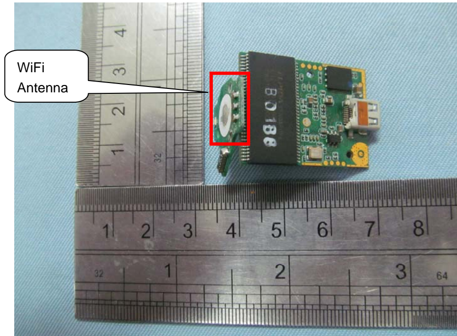
OPEN VIEW-9 OF EUT
