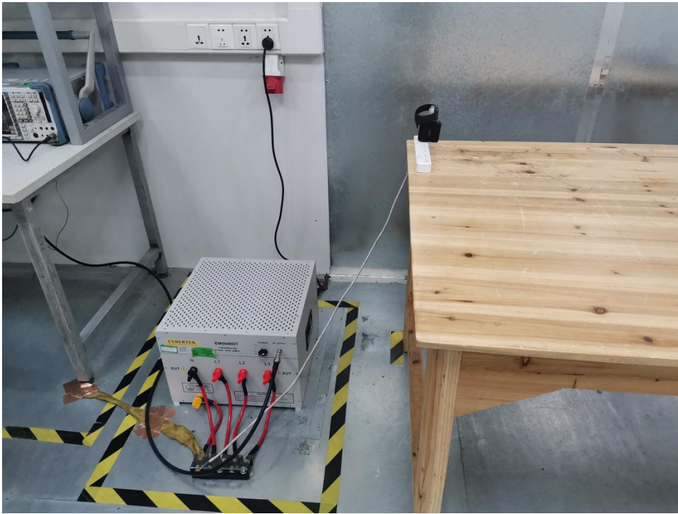
FCC ID:ZE9-ST-WMCS3MAW Photo of Conducted Emission Measurement
