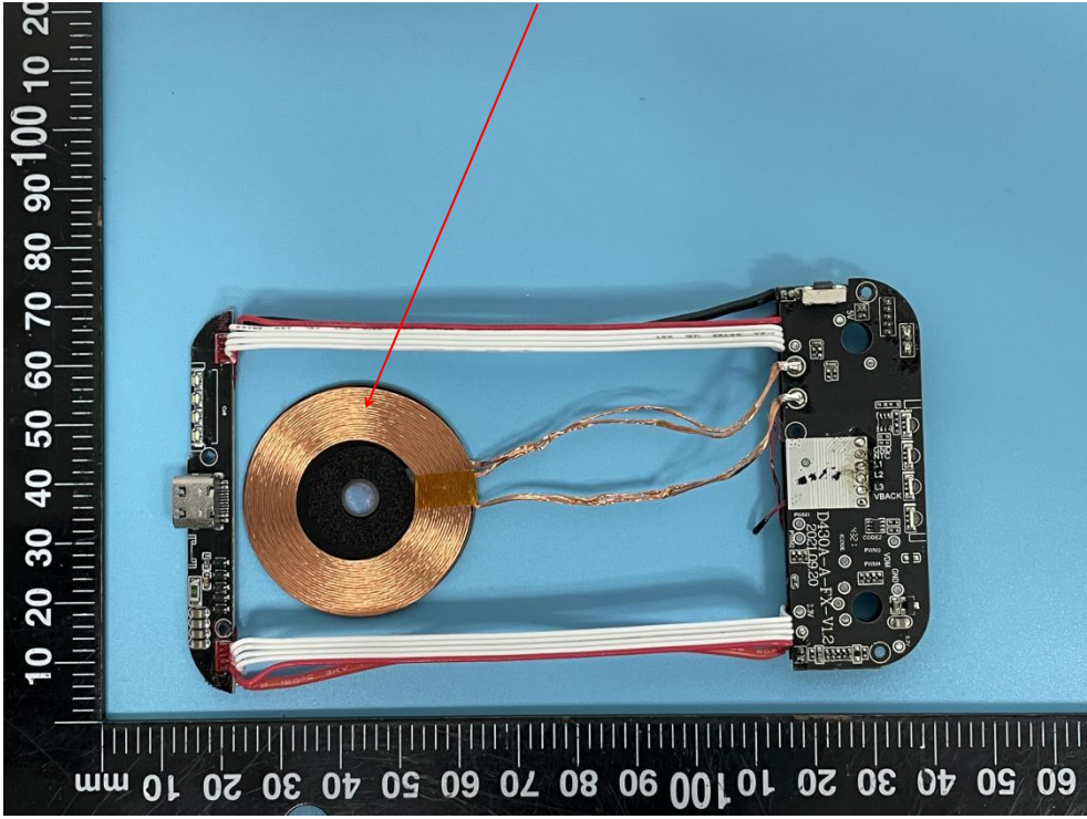
Tx Coil
