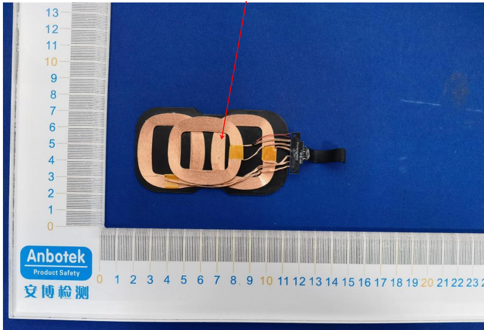
Tx Coil
