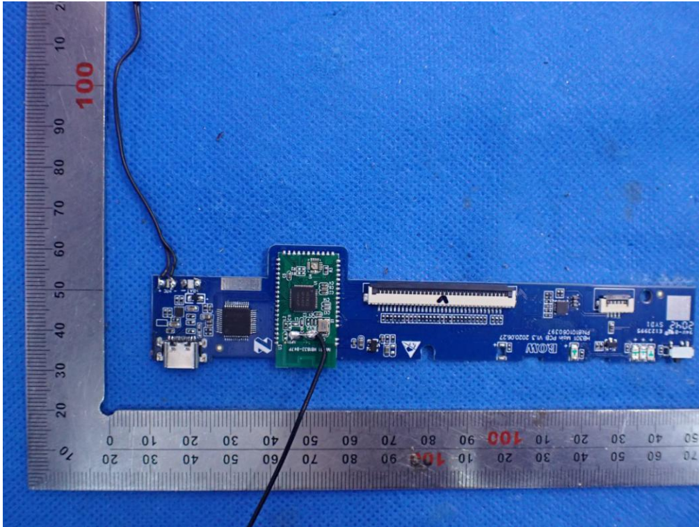
INTERNAL VIEW-4 OF EUT(ST-BTSX3)
