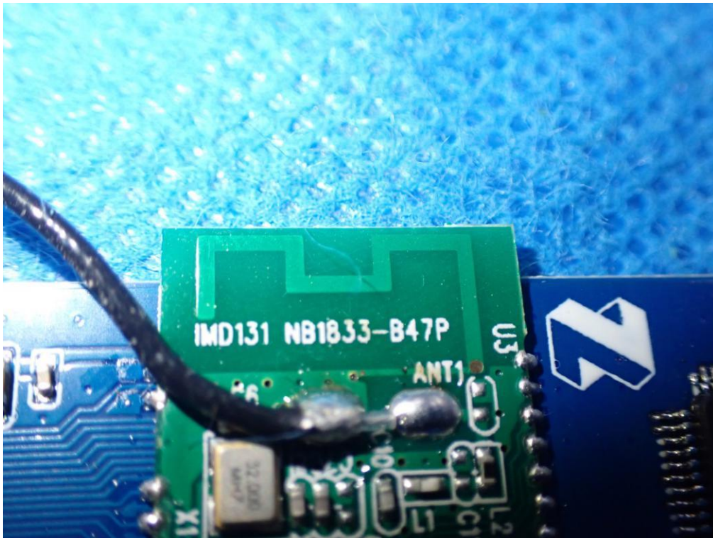
INTERNAL VIEW-6 OF EUT(ST-BTSX1)
