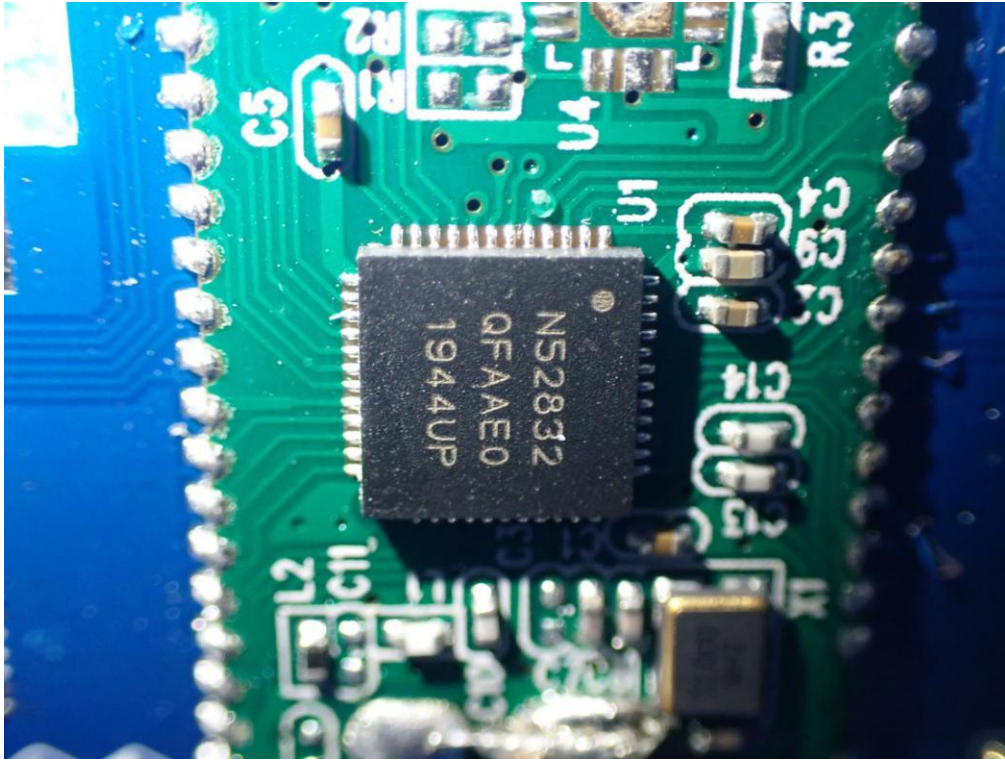
INTERNAL VIEW-6 OF EUT(ST-BTSX3)
