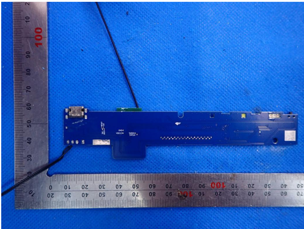
INTERNAL VIEW-4 OF EUT(ST-BTSX1)
