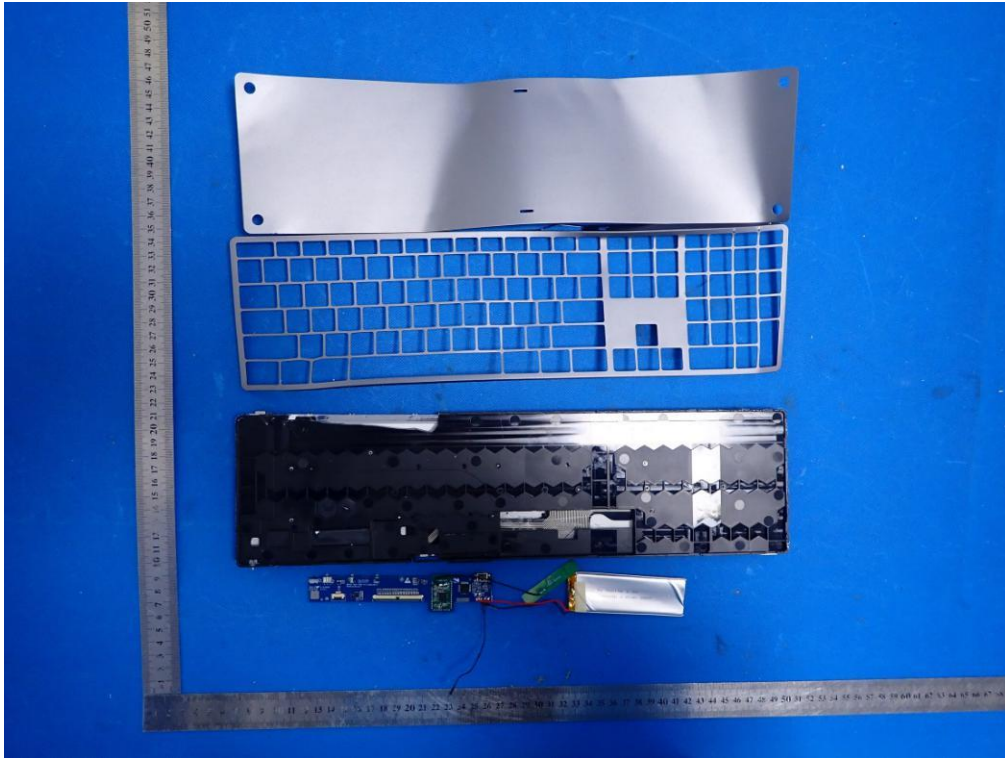
INTERNAL VIEW-2 OF EUT(ST-BTSX3)
