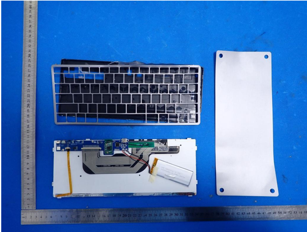
INTERNAL VIEW-2 OF EUT(ST-BTSX1)
