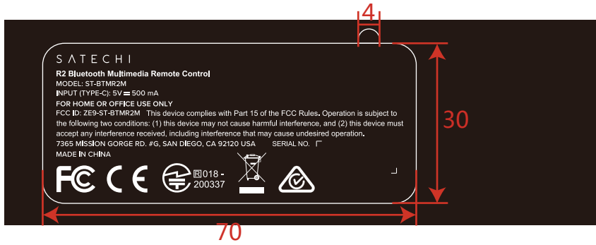
(Label location: back side of the device)
