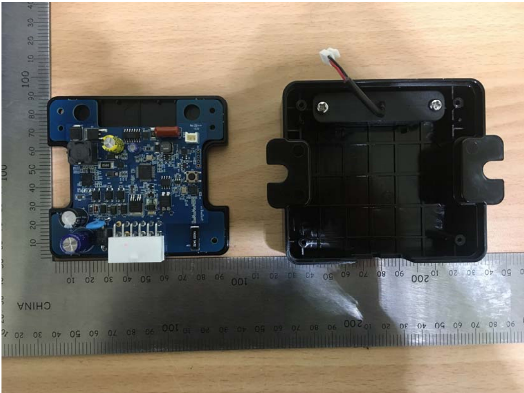
Cover opened
