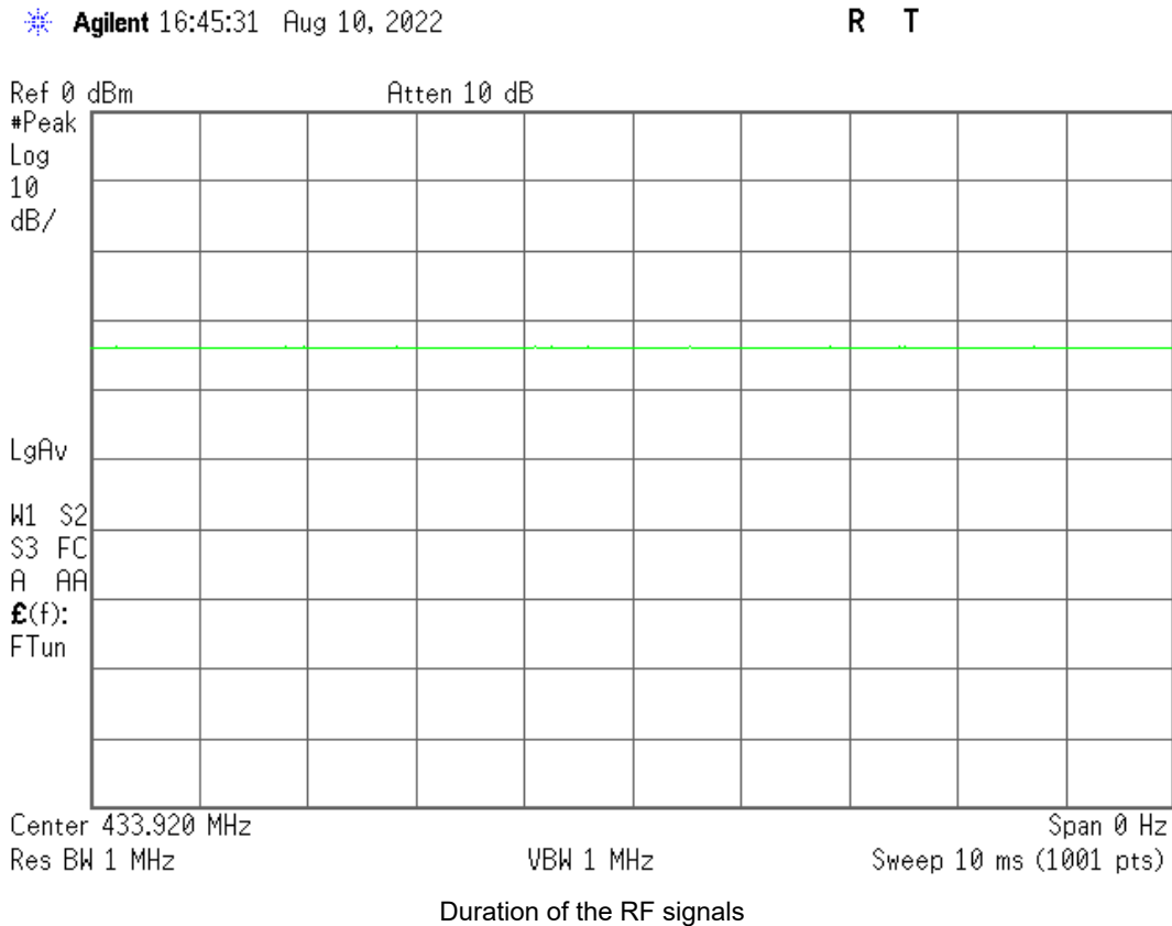
Figure 3. RF signals during the measurements achieved by the modification of firmware EUT (SAMPLE#1) firmware modification transmits a signal when the button is released RF signal has been modified to transmit continuously
