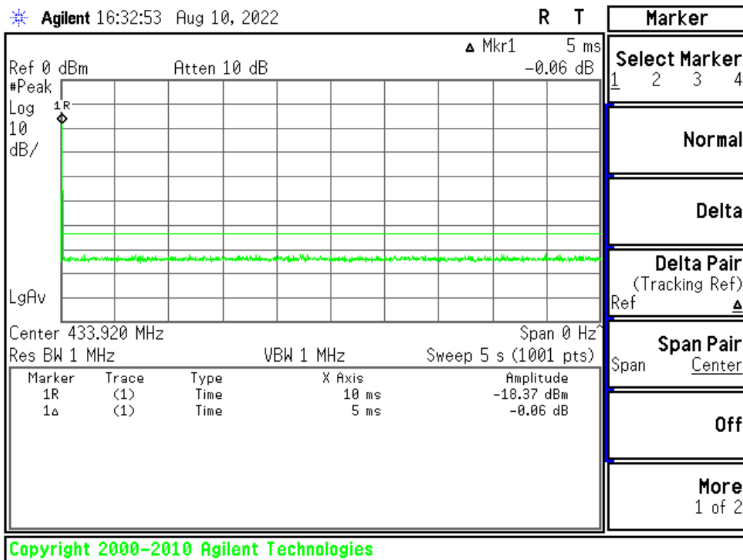
Figure 2. Plot of the Transmission Time
