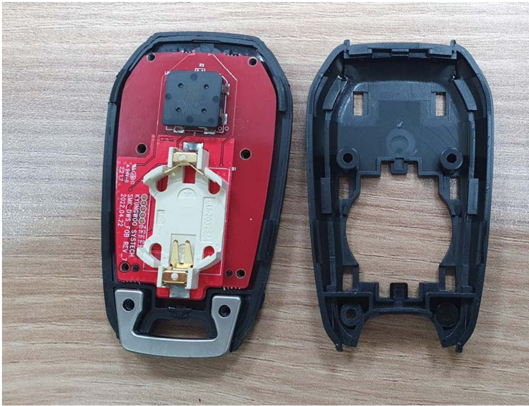
Cover opened
