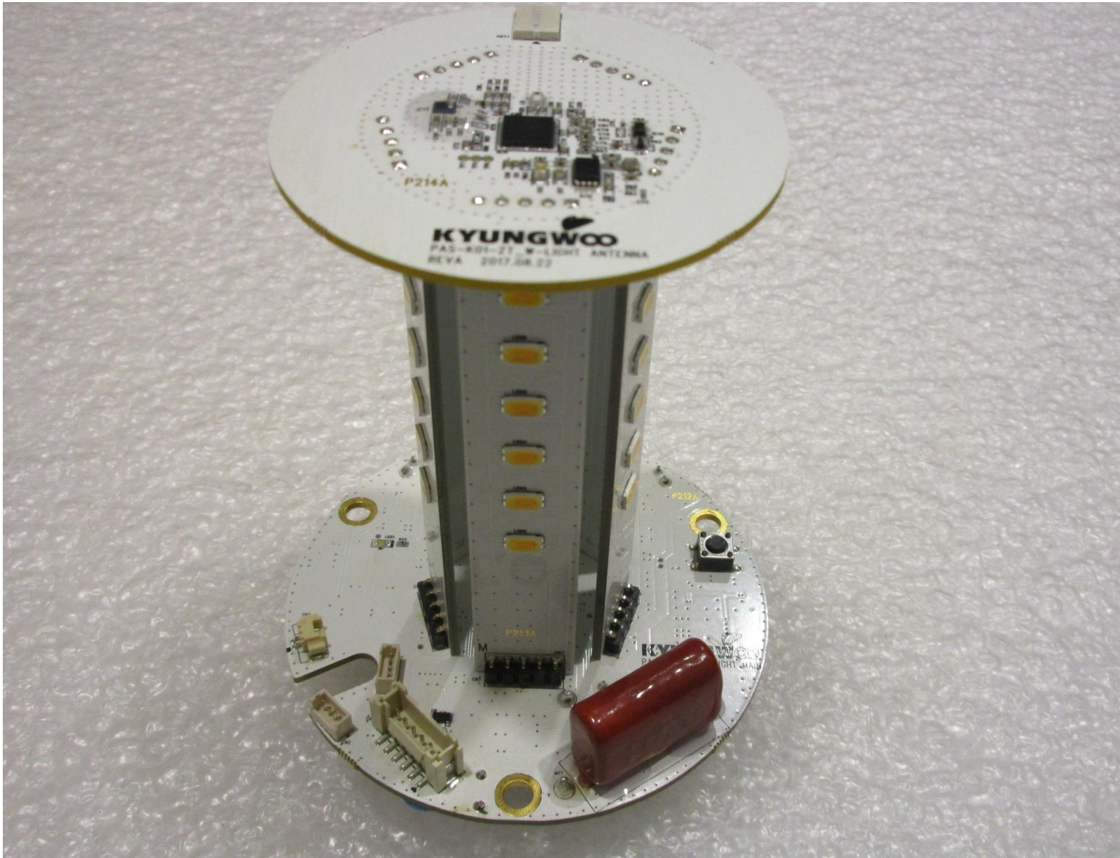
FRONT VIEW
