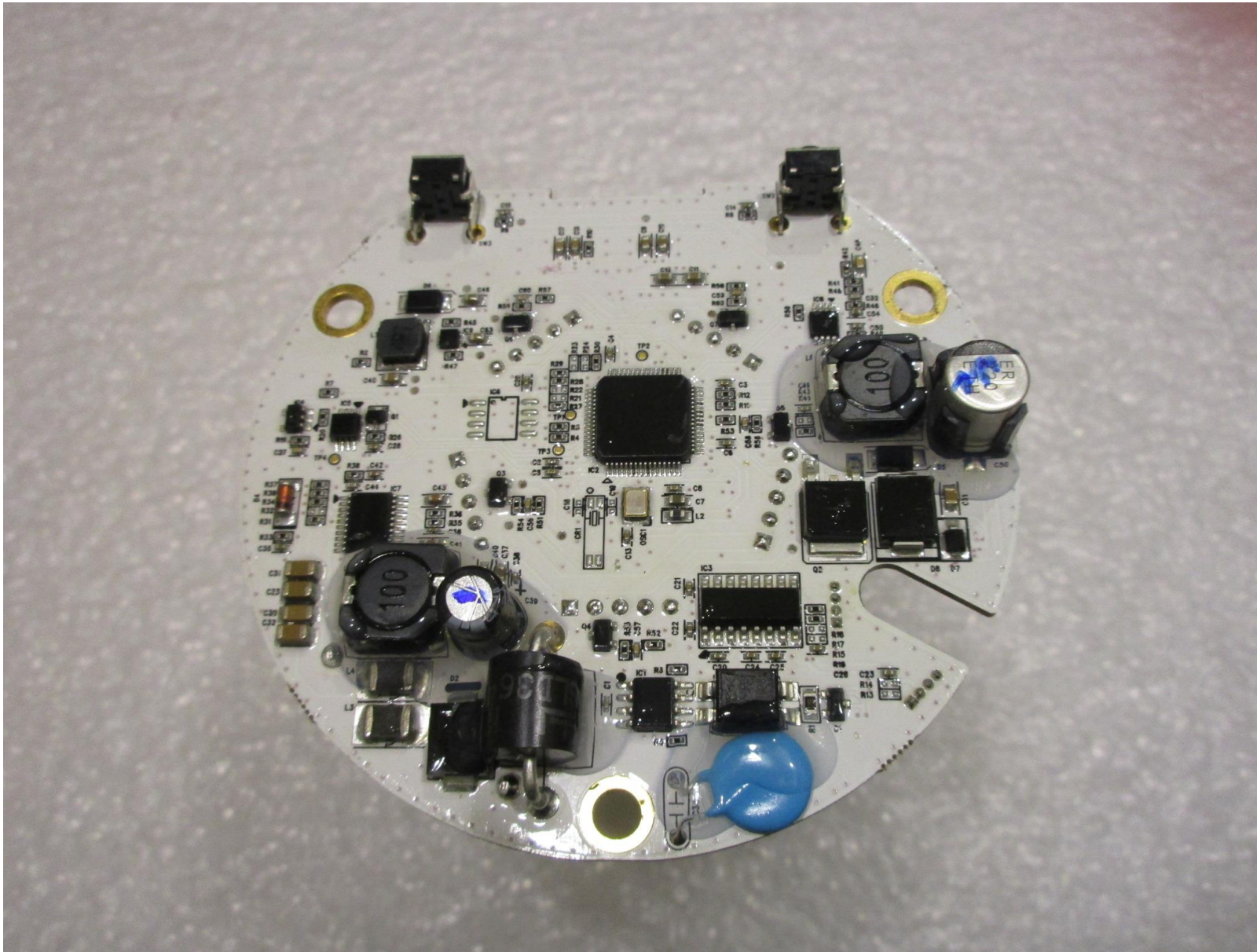
BOTTOM VIEW
