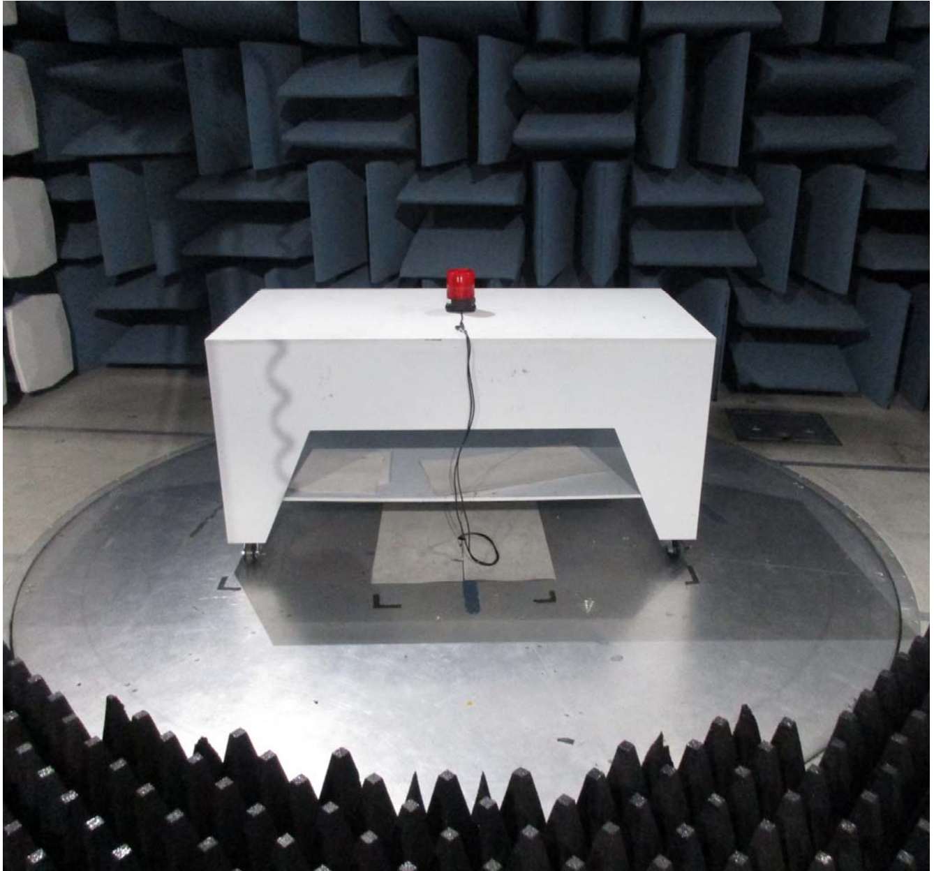
BACK VIEW FCC Class A - Radiated Emissions (>1GHz)
