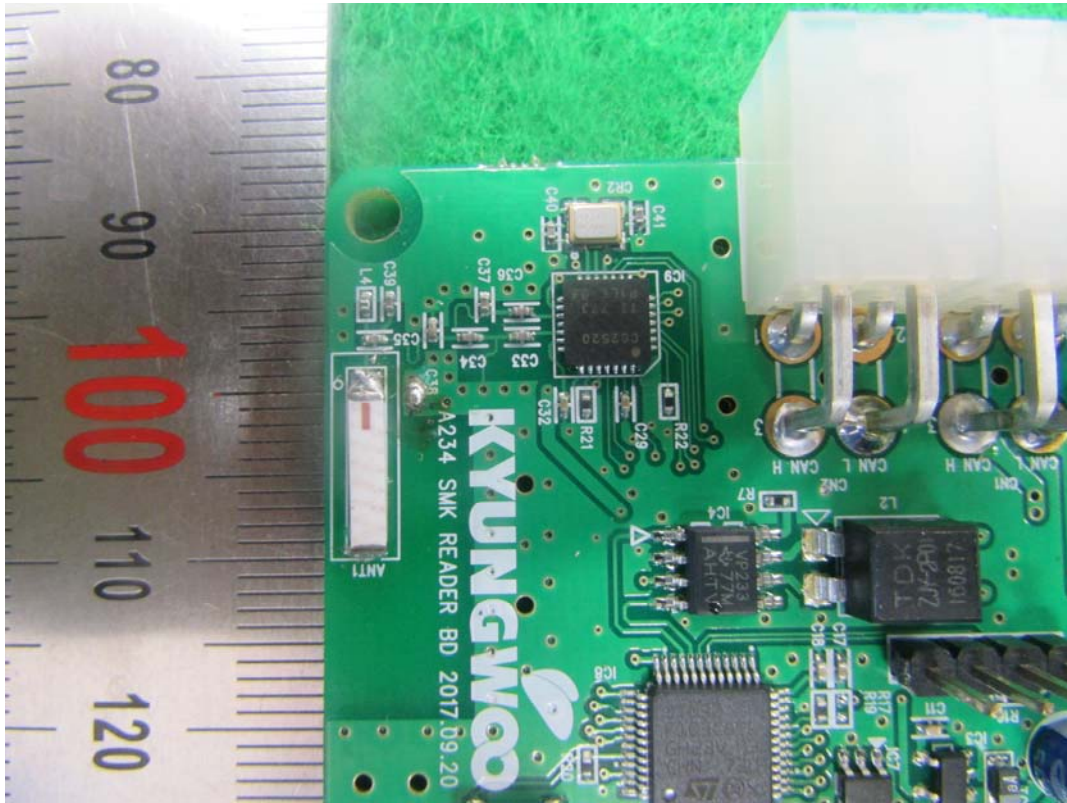
Antenna (Loop Coil antenna for 125 kHz Transmitter)
