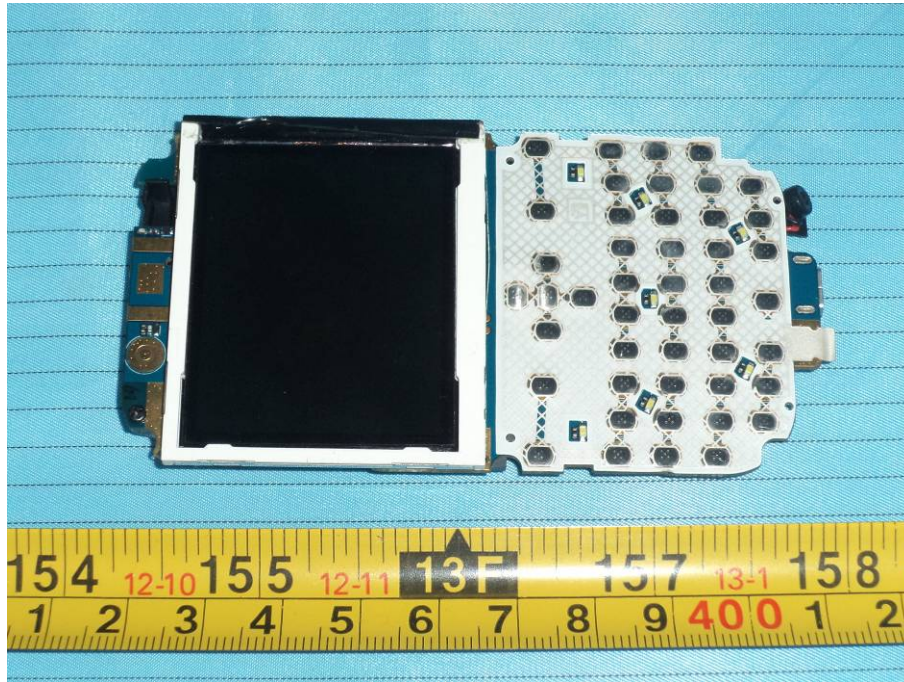
EUT – Main Board with LCD and Keyboard Bottom View
