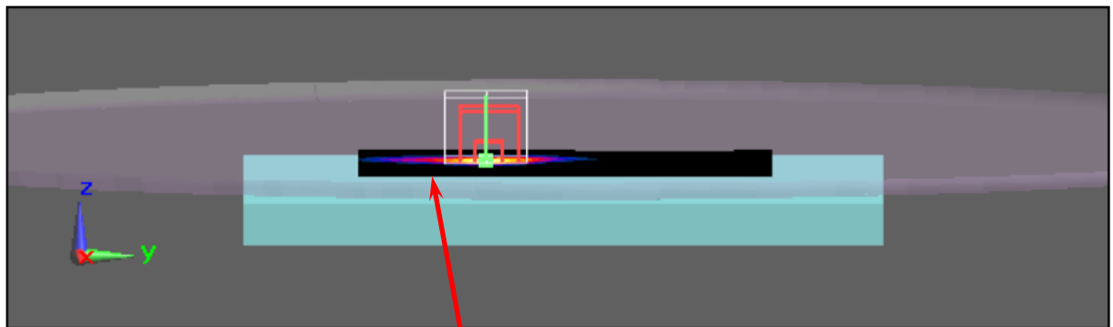
Figure 1. Body SAR Test Setup (Flat Section) Back surface to phantom 0mm
