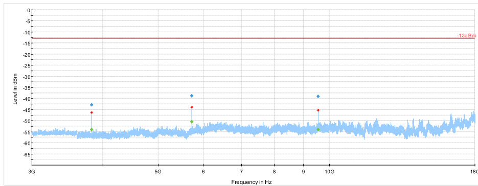
Preview Result 1-PK+ Critical_Freqs PK+ -13dBm Final_Result PK+ Final_Result RMS
