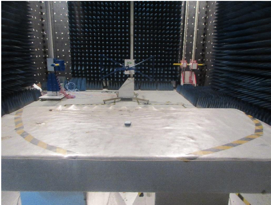
DTS_DXX radiation L
