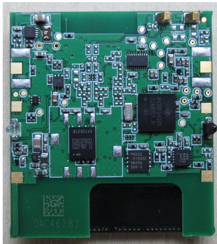
Figure 2: Smart TAG PCB, bottom
