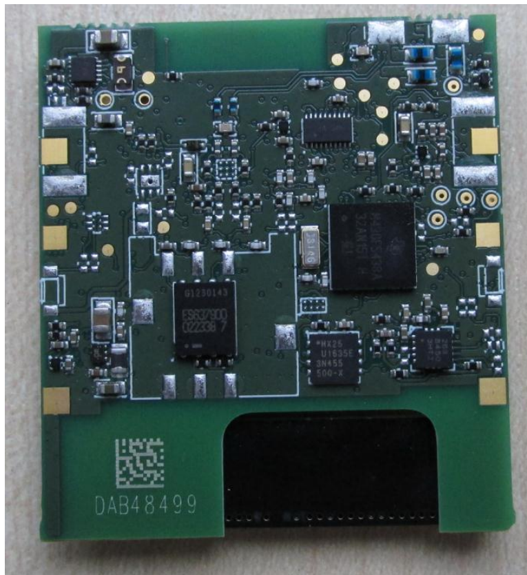
Figure 2: main PCB, bottom
