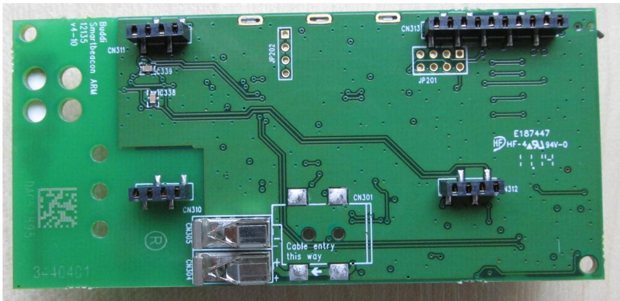
Figure 3: ARM (peripheral) board, top
