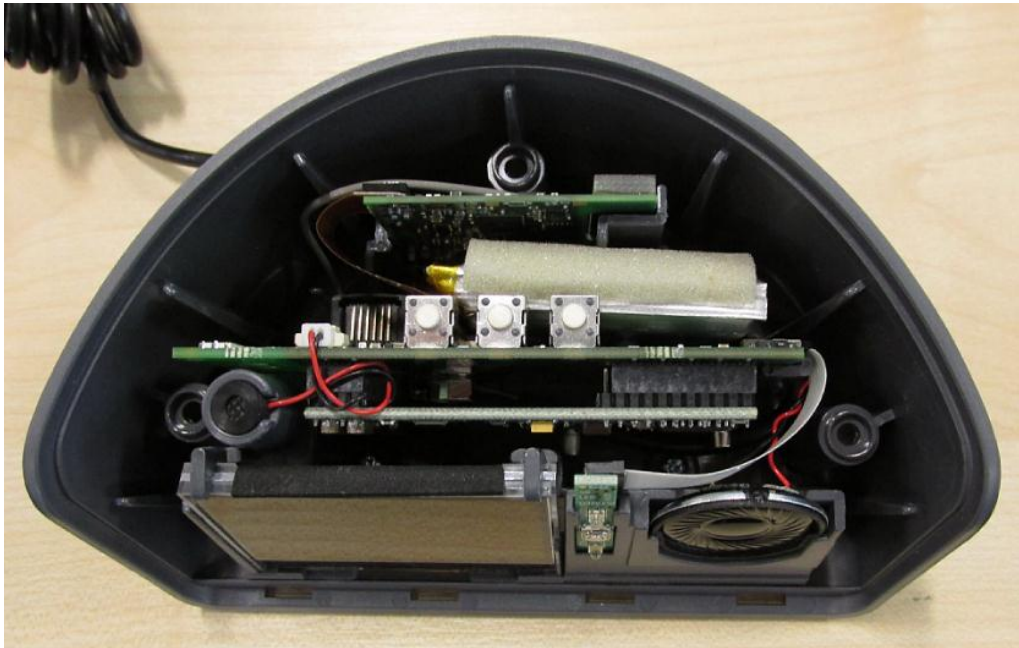
Figure 7: Smart Beacon internals, with landline modem
