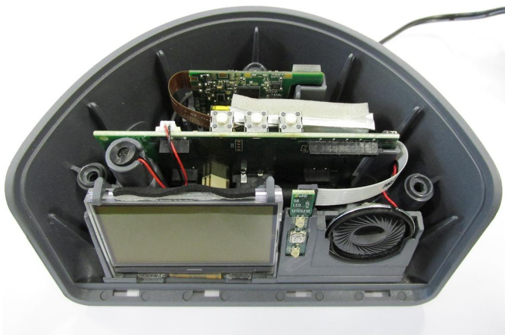
Figure 6: Smart Beacon internal, without landline modem
