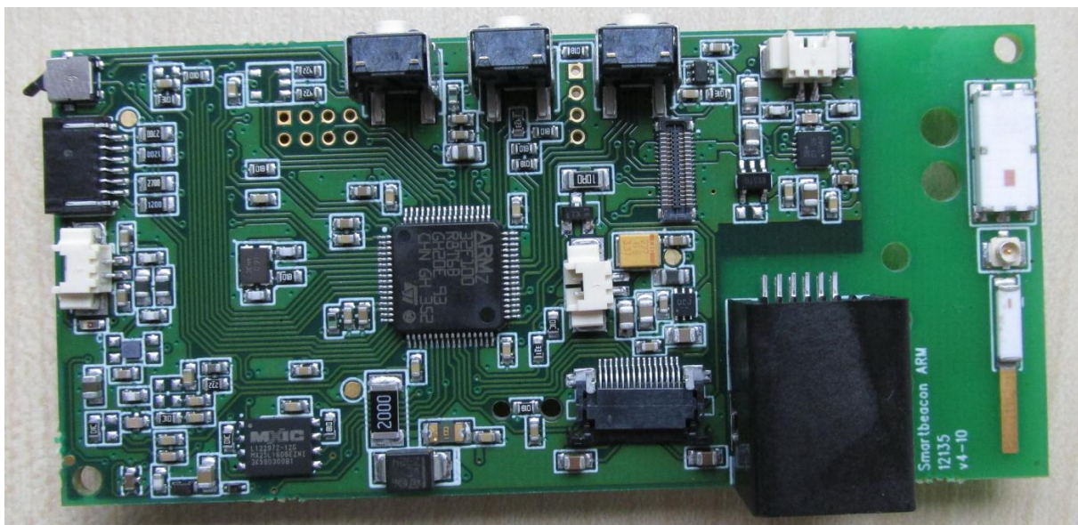
Figure 4: ARM (peripheral) board, bottom
