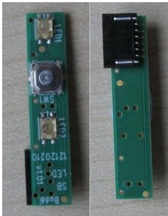
Figure 5: LED board, TOP and bottom
