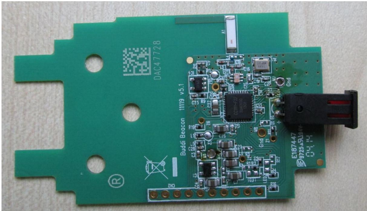
Figure 1: RF Beacon PCB, top
