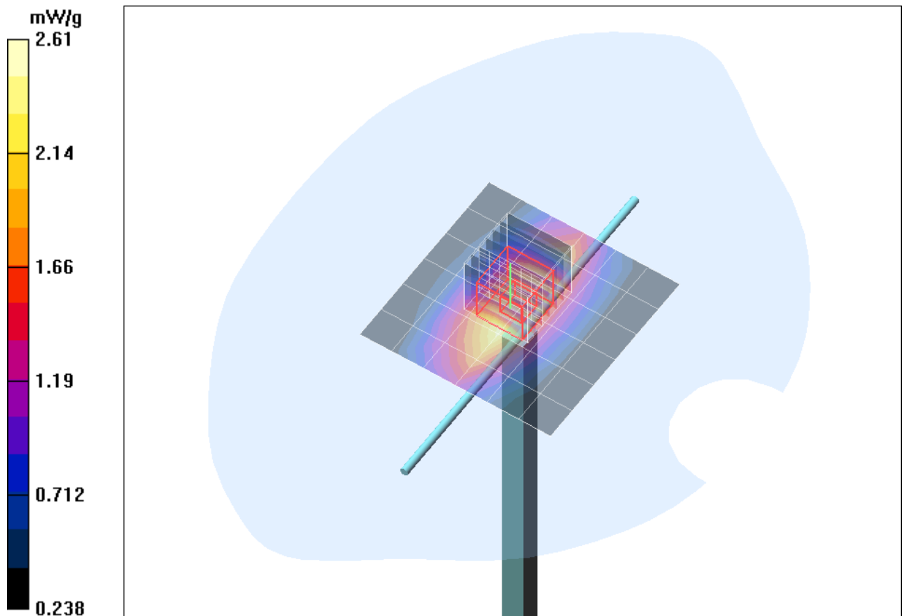
Fig. 10: Validation measurement 835 MHz Body (March 29, 2011), coarse grid. Ambient Temperature: 20.8°C, Liquid Temperature: 20.3°C.
